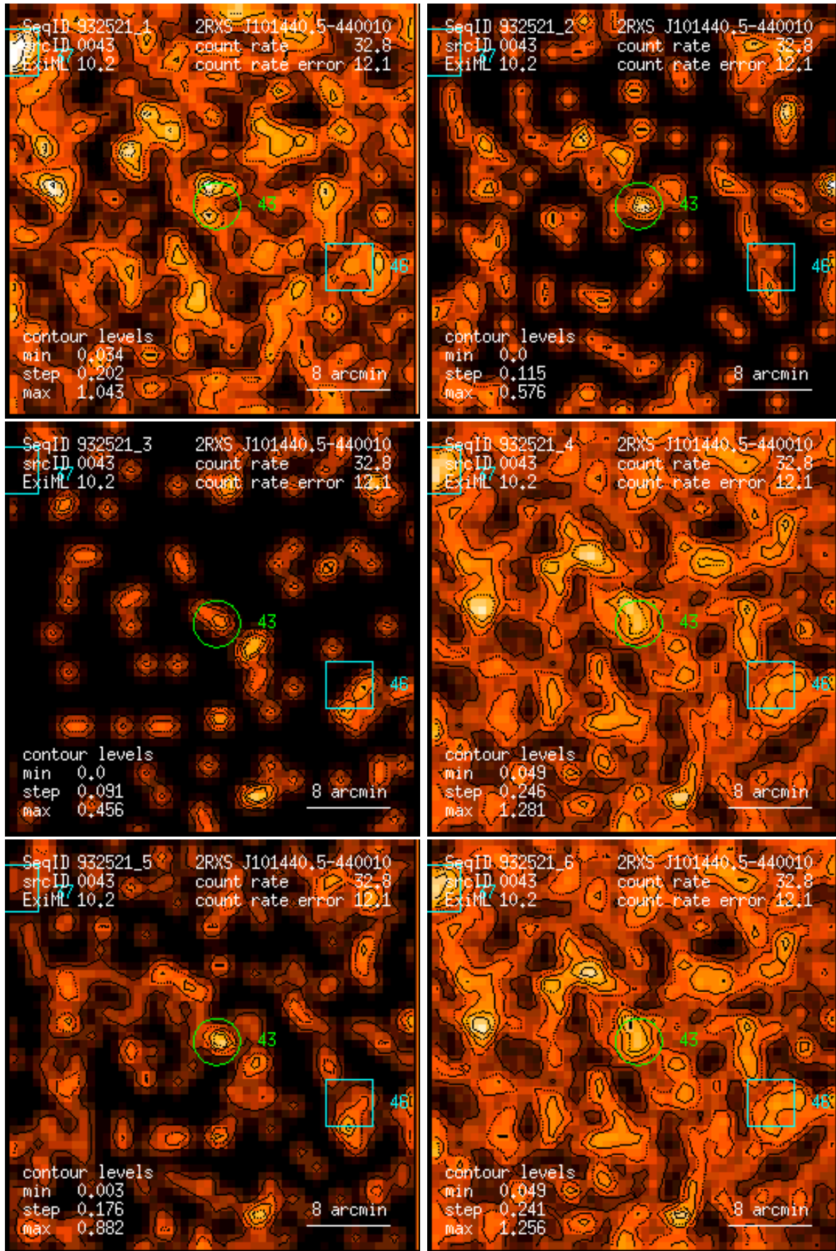
Figure 43: RASS 932521: detection 0043: band rate images, Gaussian filter: (1) PSPC channels 11 – 41, (2) 52 – 90, (3) 91 – 201, (4) 11 – 235, (5) 52 – 201, (6) 11 – 201. Broad band rates in counts/ks. Band rate contour levels in counts/ks/arcmin 2 .
