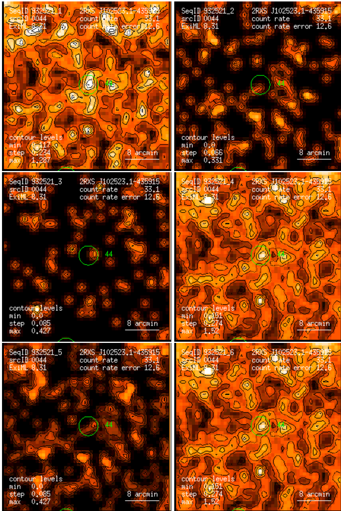
Figure 44: RASS 932521: detection 0044: band rate images, Gaussian filter: (1) PSPC channels 11 – 41, (2) 52 – 90, (3) 91 – 201, (4) 11 – 235, (5) 52 – 201, (6) 11 – 201. Broad band rates in counts/ks. Band rate contour levels in counts/ks/arcmin 2 .
