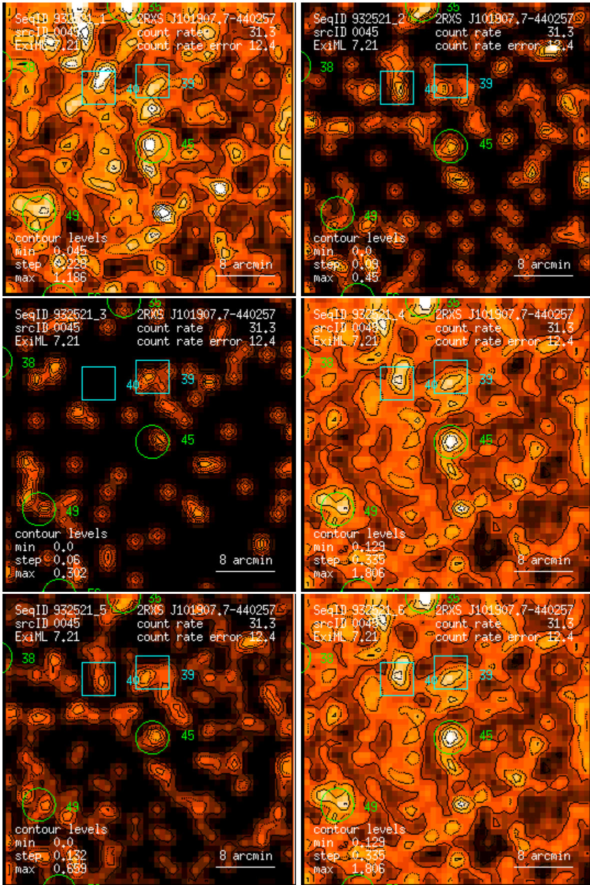
Figure 45: RASS 932521: detection 0045: band rate images, Gaussian filter: (1) PSPC channels 11 – 41, (2) 52 – 90, (3) 91 – 201, (4) 11 – 235, (5) 52 – 201, (6) 11 – 201. Broad band rates in counts/ks. Band rate contour levels in counts/ks/arcmin 2 .
