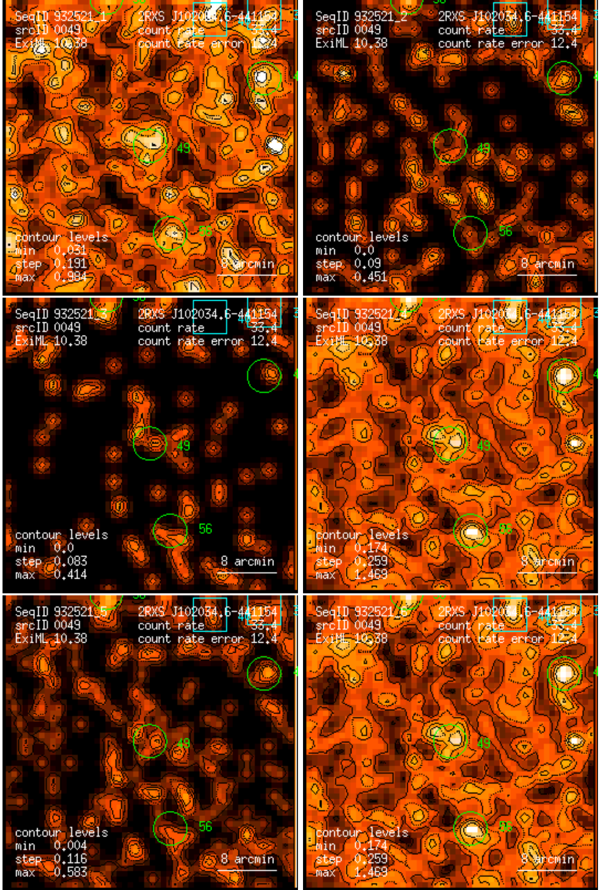
Figure 49: RASS 932521: detection 0049: band rate images, Gaussian filter: (1) PSPC channels 11 – 41, (2) 52 – 90, (3) 91 – 201, (4) 11 – 235, (5) 52 – 201, (6) 11 – 201. Broad band rates in counts/ks. Band rate contour levels in counts/ks/arcmin 2 .
