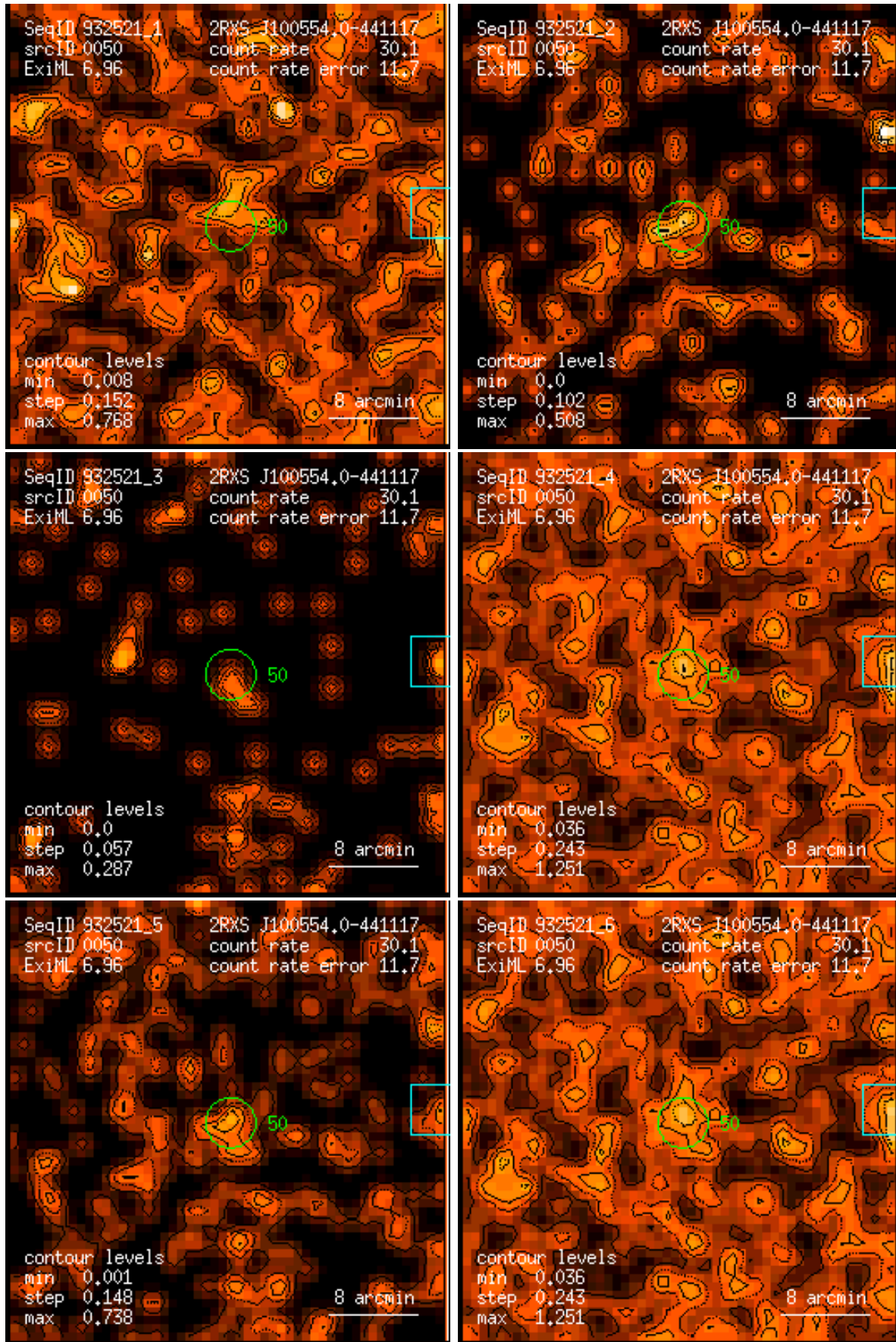
Figure 50: RASS 932521: detection 0050: band rate images, Gaussian filter: (1) PSPC channels 11 – 41, (2) 52 – 90, (3) 91 – 201, (4) 11 – 235, (5) 52 – 201, (6) 11 – 201. Broad band rates in counts/ks. Band rate contour levels in counts/ks/arcmin 2 .
