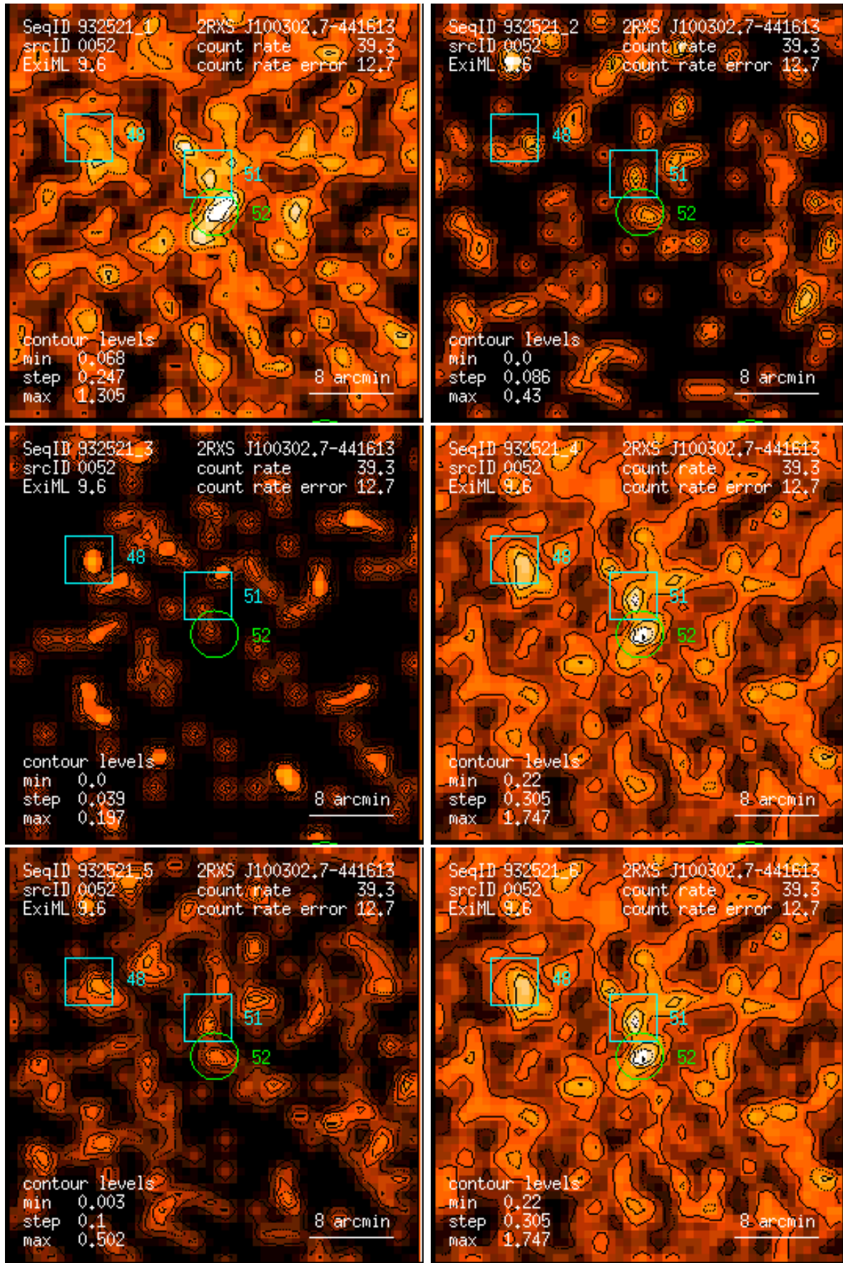
Figure 52: RASS 932521: detection 0052: band rate images, Gaussian filter: (1) PSPC channels 11 – 41, (2) 52 – 90, (3) 91 – 201, (4) 11 – 235, (5) 52 – 201, (6) 11 – 201. Broad band rates in counts/ks. Band rate contour levels in counts/ks/arcmin 2 .
