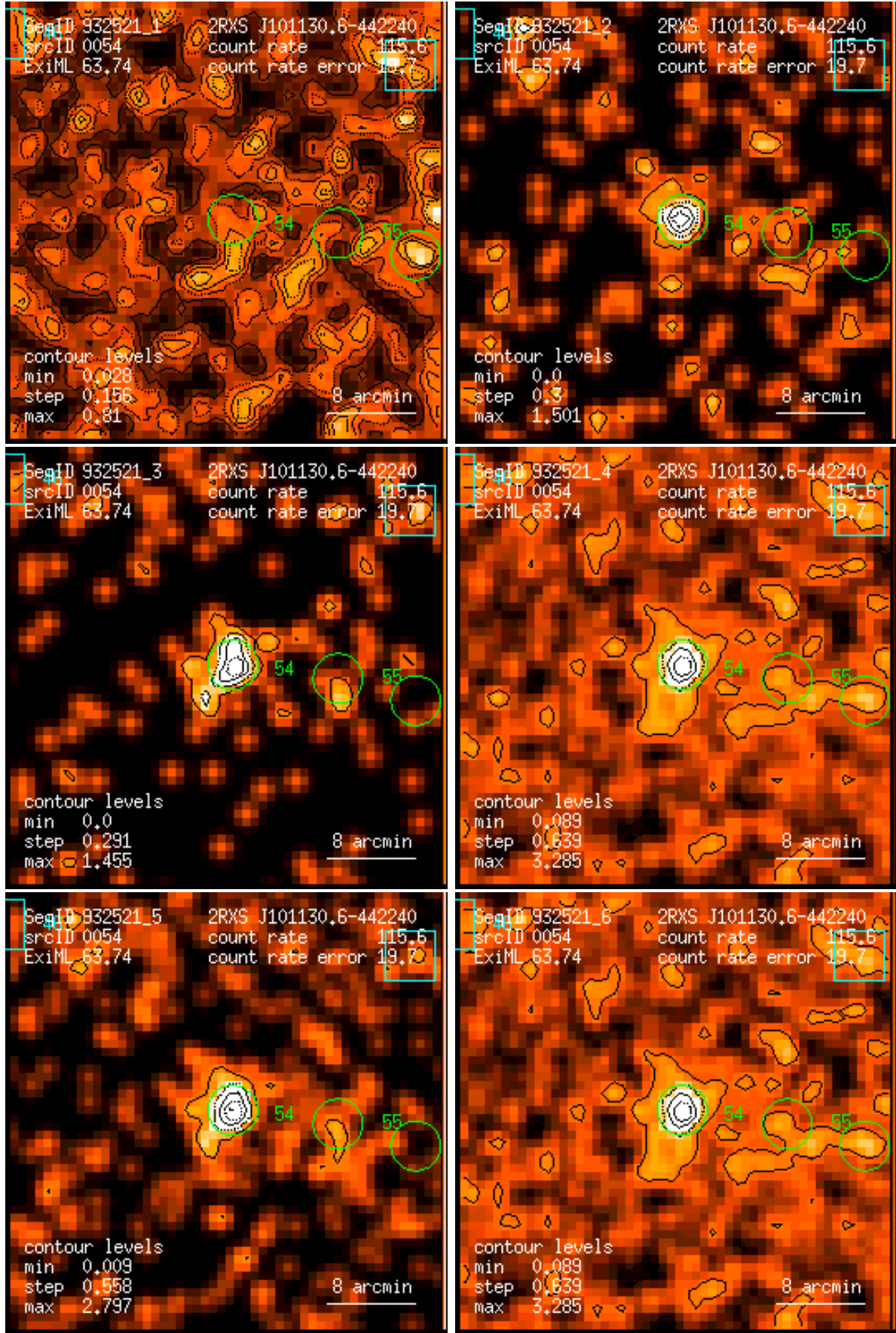
Figure 54: RASS 932521: detection 0054: band rate images, Gaussian filter: (1) PSPC channels 11 – 41, (2) 52 – 90, (3) 91 – 201, (4) 11 – 235, (5) 52 – 201, (6) 11 – 201. Broad band rates in counts/ks. Band rate contour levels in counts/ks/arcmin 2 .
