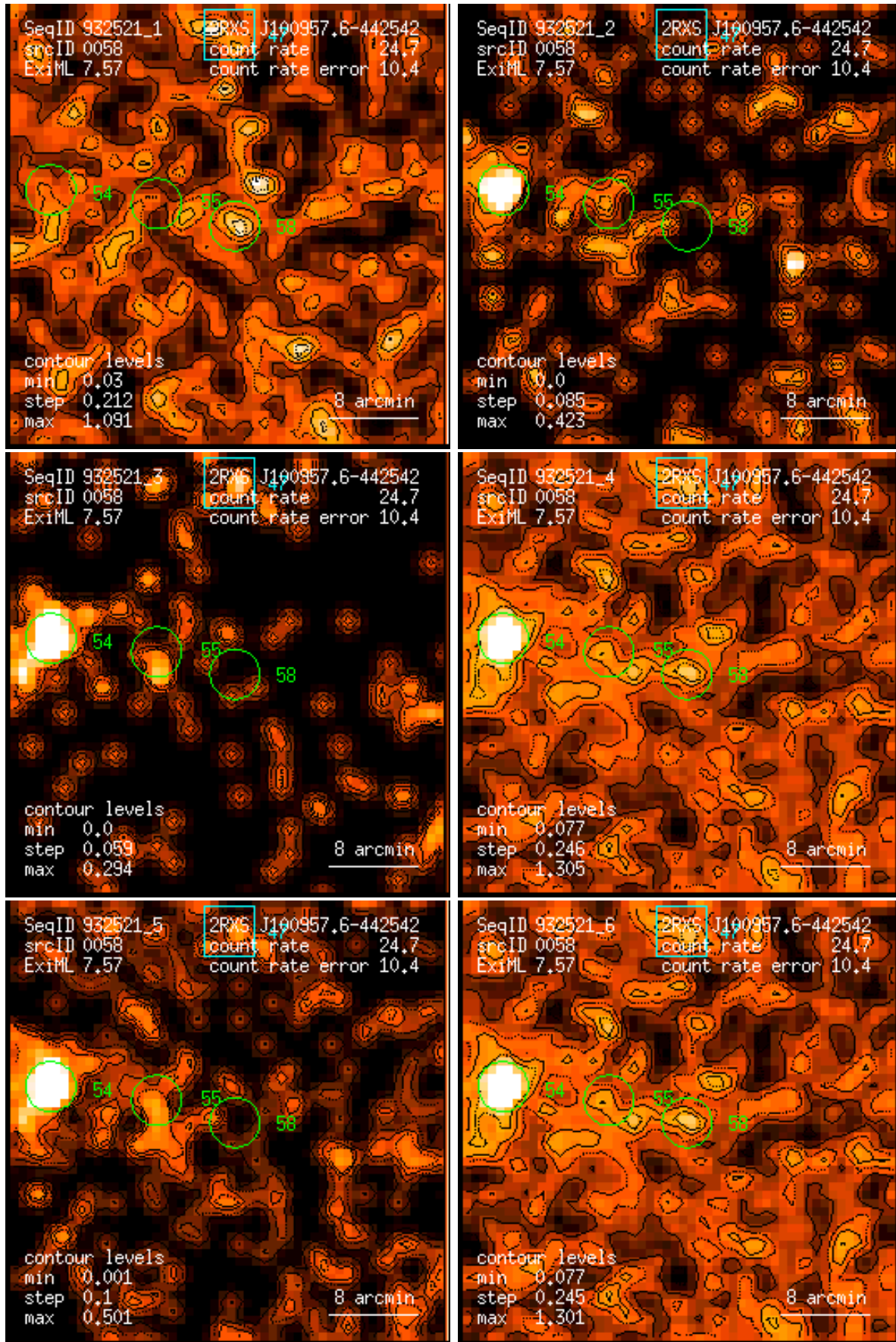
Figure 58: RASS 932521: detection 0058: band rate images, Gaussian filter: (1) PSPC channels 11 – 41, (2) 52 – 90, (3) 91 – 201, (4) 11 – 235, (5) 52 – 201, (6) 11 – 201. Broad band rates in counts/ks. Band rate contour levels in counts/ks/arcmin 2 .
