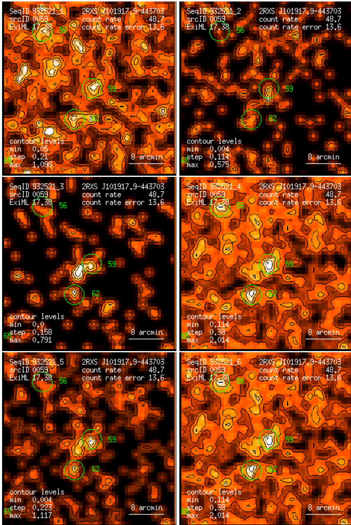
Figure 59: RASS 932521: detection 0059: band rate images, Gaussian filter: (1) PSPC channels 11 – 41, (2) 52 – 90, (3) 91 – 201, (4) 11 – 235, (5) 52 – 201, (6) 11 – 201. Broad band rates in counts/ks. Band rate contour levels in counts/ks/arcmin 2 .
