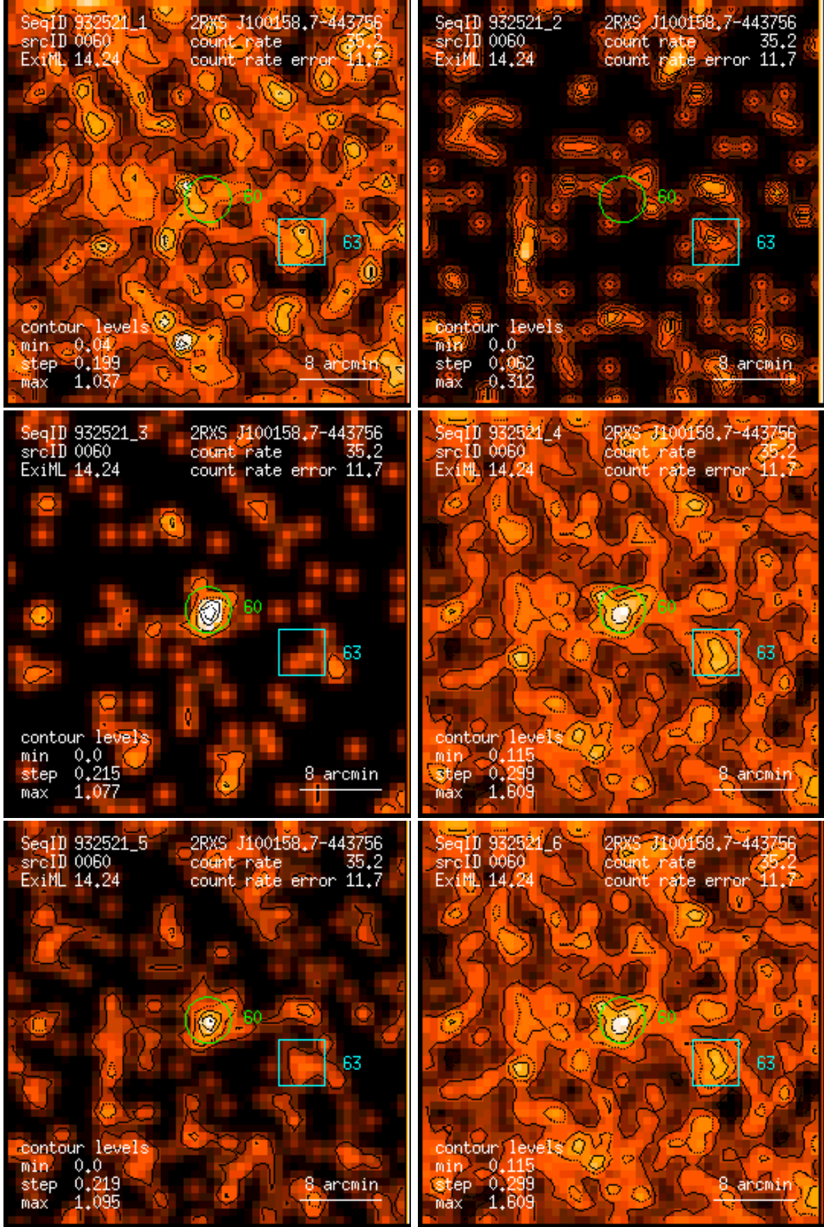
Figure 60: RASS 932521: detection 0060: band rate images, Gaussian filter: (1) PSPC channels 11 – 41, (2) 52 – 90, (3) 91 – 201, (4) 11 – 235, (5) 52 – 201, (6) 11 – 201. Broad band rates in counts/ks. Band rate contour levels in counts/ks/arcmin 2 .
