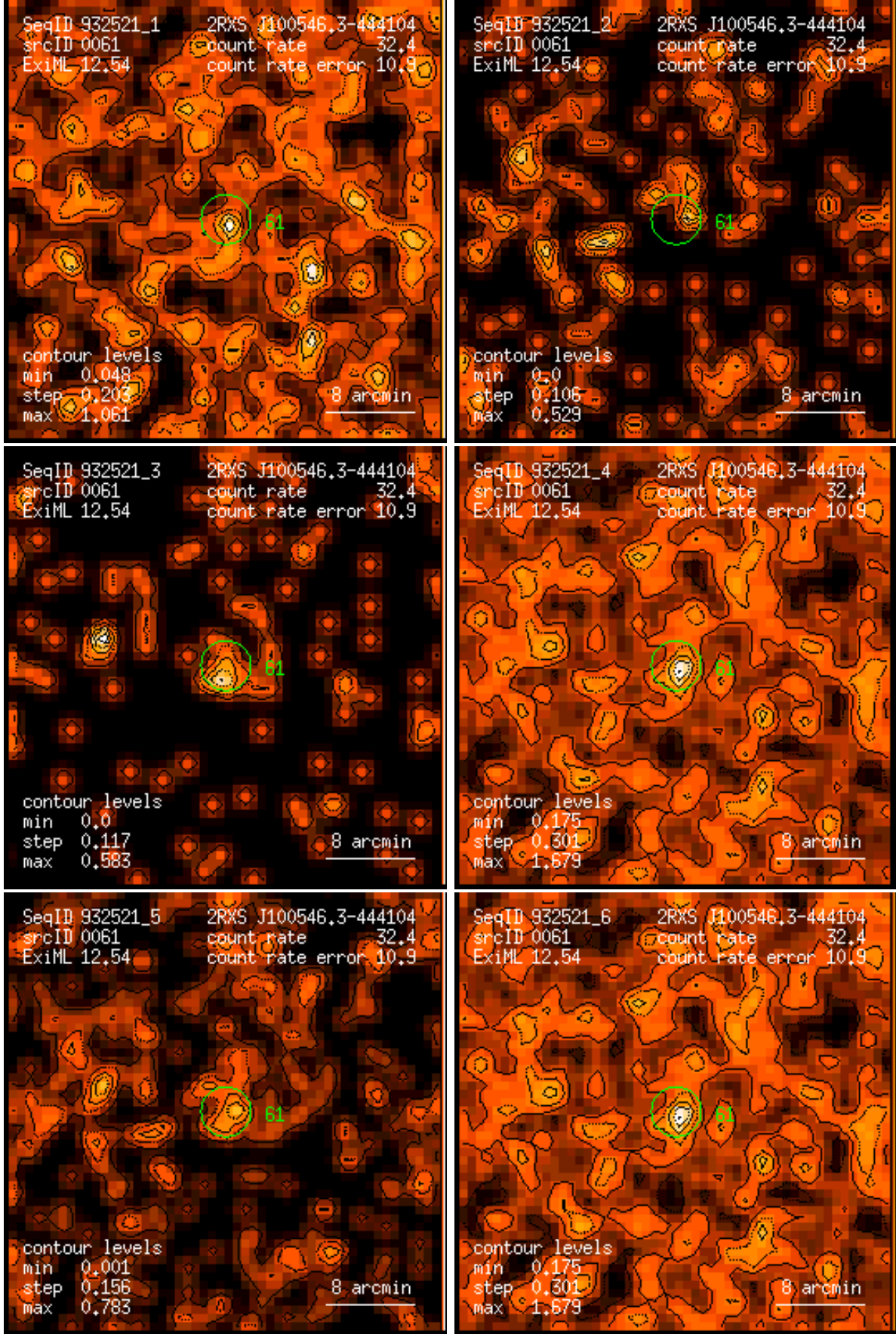
Figure 61: RASS 932521: detection 0061: band rate images, Gaussian filter: (1) PSPC channels 11 – 41, (2) 52 – 90, (3) 91 – 201, (4) 11 – 235, (5) 52 – 201, (6) 11 – 201. Broad band rates in counts/ks. Band rate contour levels in counts/ks/arcmin 2 .
