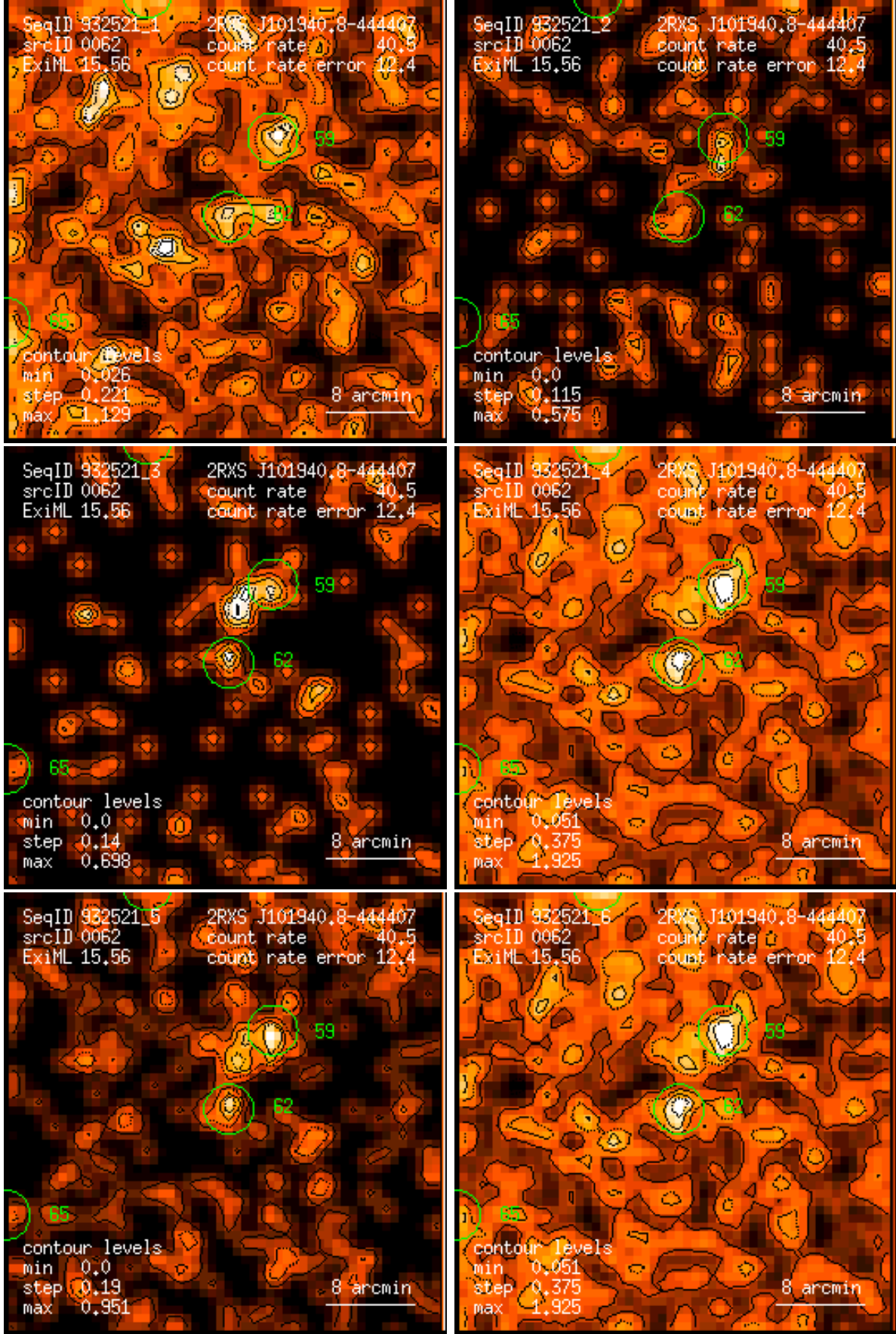
Figure 62: RASS 932521: detection 0062: band rate images, Gaussian filter: (1) PSPC channels 11 – 41, (2) 52 – 90, (3) 91 – 201, (4) 11 – 235, (5) 52 – 201, (6) 11 – 201. Broad band rates in counts/ks. Band rate contour levels in counts/ks/arcmin 2 .
