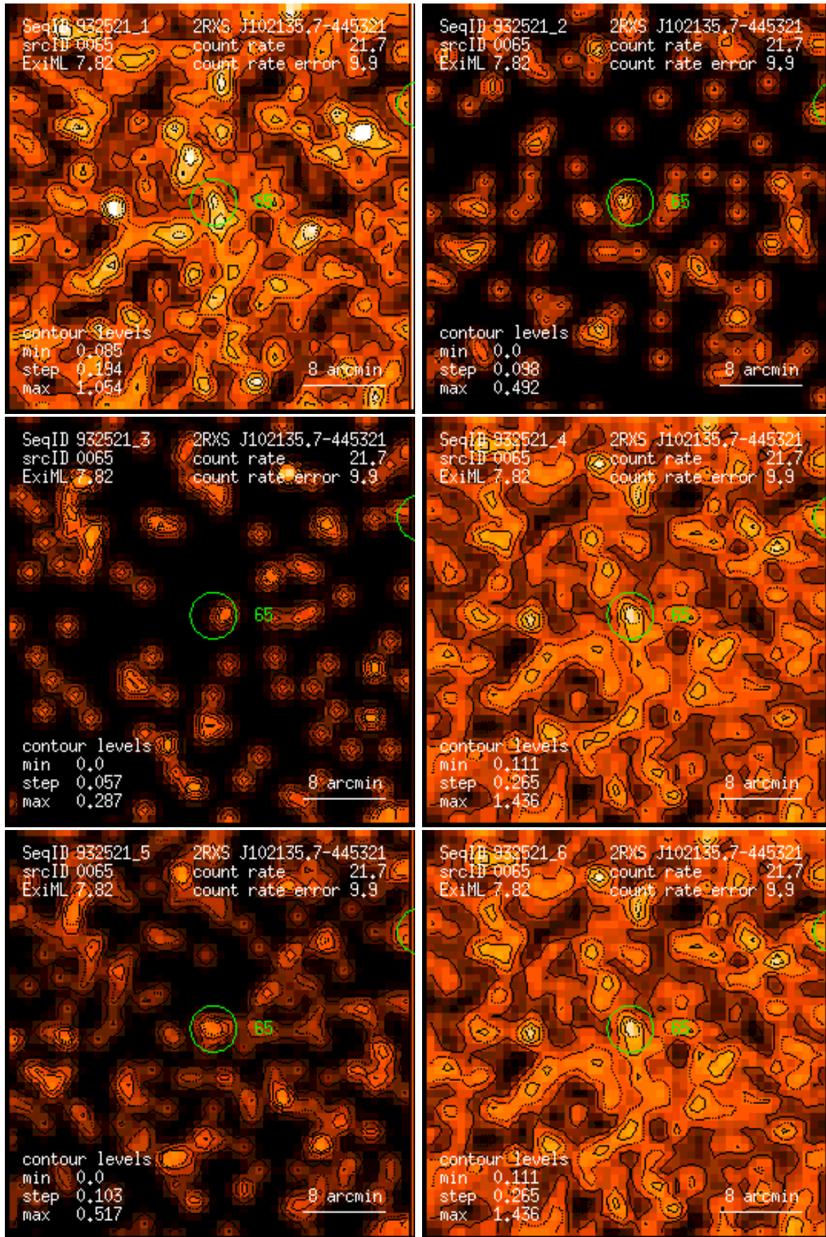
Figure 65: RASS 932521: detection 0065: band rate images, Gaussian filter: (1) PSPC channels 11 – 41, (2) 52 – 90, (3) 91 – 201, (4) 11 – 235, (5) 52 – 201, (6) 11 – 201. Broad band rates in counts/ks. Band rate contour levels in counts/ks/arcmin 2 .
