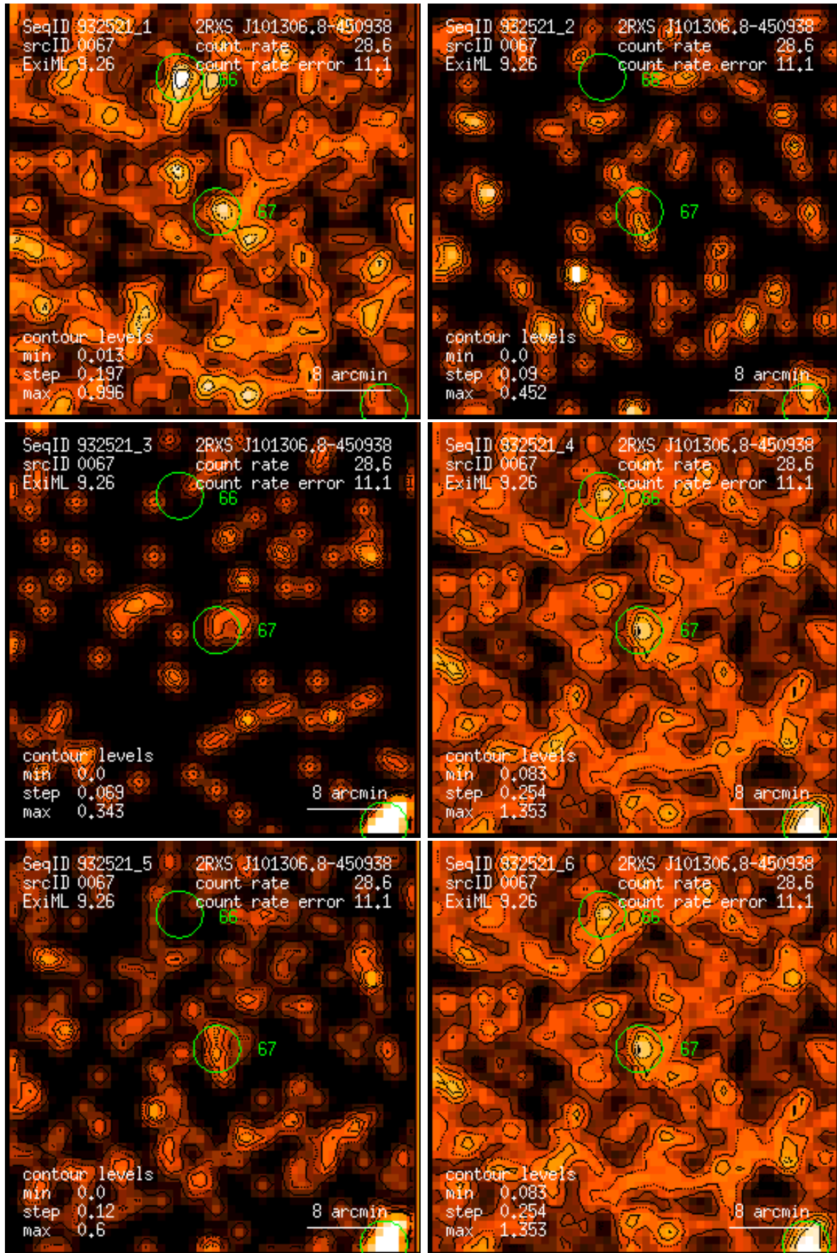
Figure 67: RASS 932521: detection 0067: band rate images, Gaussian filter: (1) PSPC channels 11 – 41, (2) 52 – 90, (3) 91 – 201, (4) 11 – 235, (5) 52 – 201, (6) 11 – 201. Broad band rates in counts/ks. Band rate contour levels in counts/ks/arcmin 2 .
