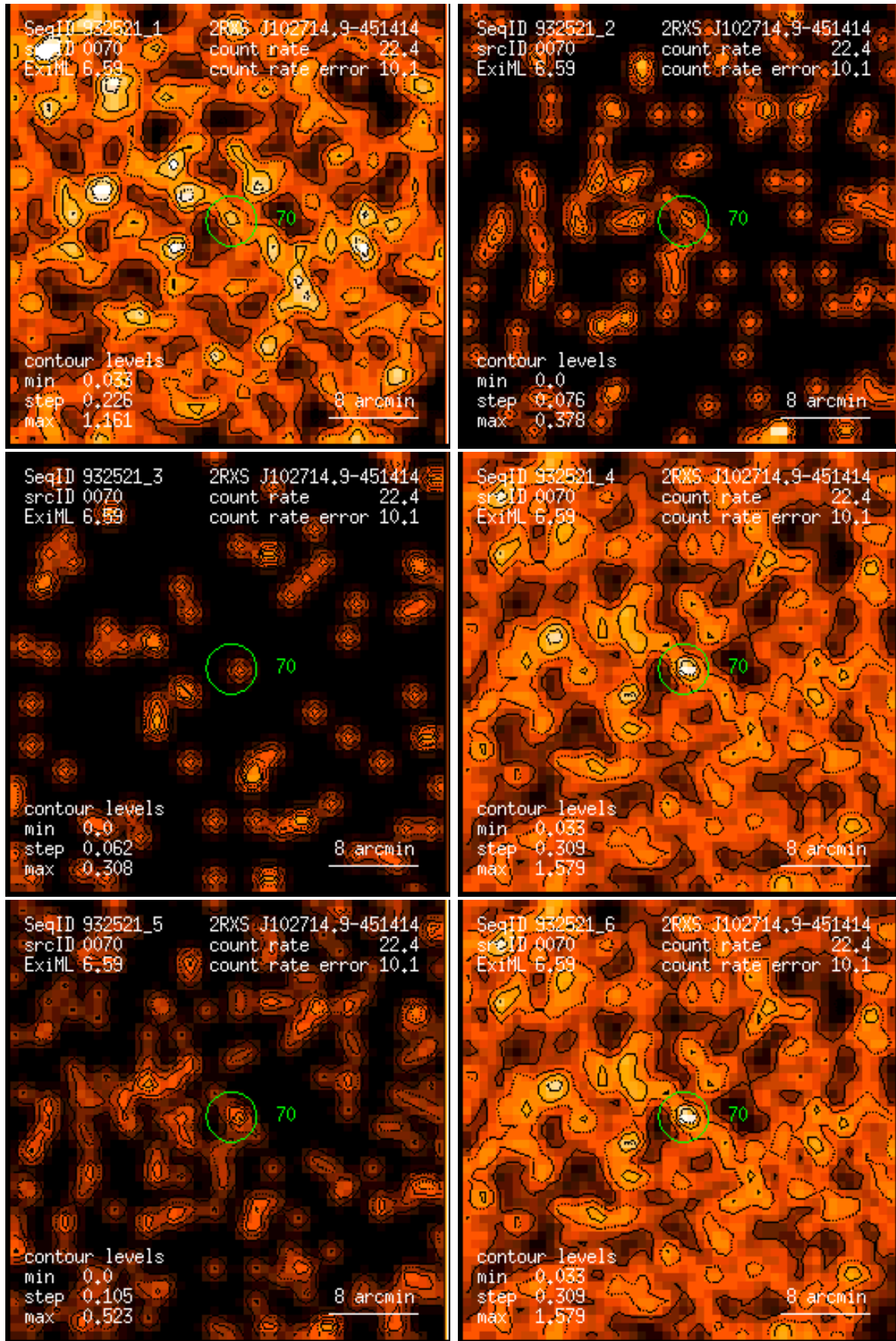
Figure 70: RASS 932521: detection 0070: band rate images, Gaussian filter: (1) PSPC channels 11 – 41, (2) 52 – 90, (3) 91 – 201, (4) 11 – 235, (5) 52 – 201, (6) 11 – 201. Broad band rates in counts/ks. Band rate contour levels in counts/ks/arcmin 2 .
