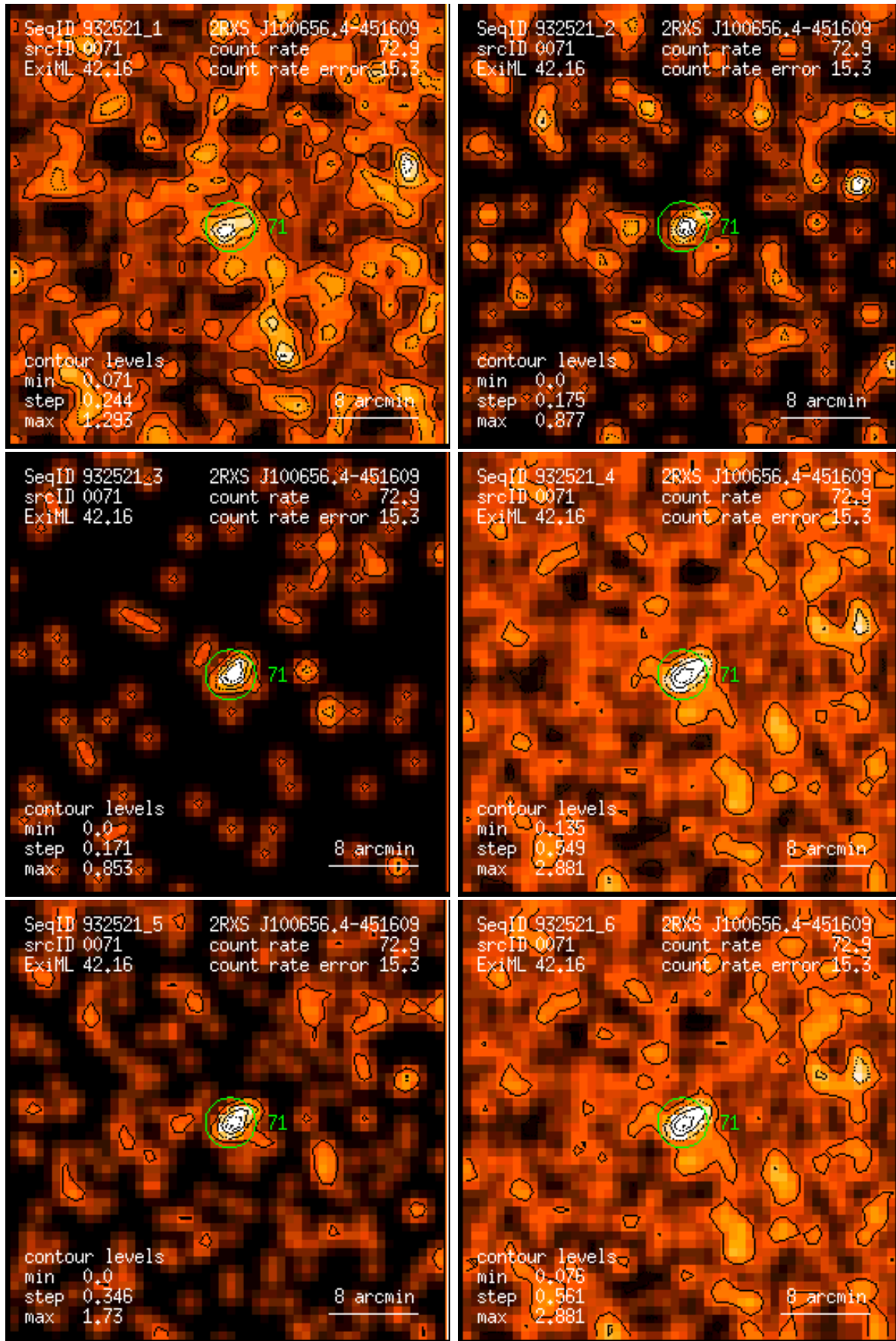
Figure 71: RASS 932521: detection 0071: band rate images, Gaussian filter: (1) PSPC channels 11 – 41, (2) 52 – 90, (3) 91 – 201, (4) 11 – 235, (5) 52 – 201, (6) 11 – 201. Broad band rates in counts/ks. Band rate contour levels in counts/ks/arcmin 2 .
