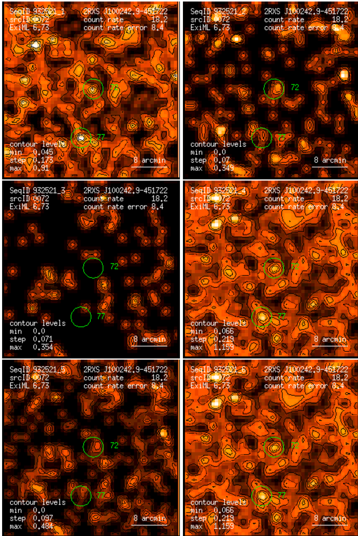
Figure 72: RASS 932521: detection 0072: band rate images, Gaussian filter: (1) PSPC channels 11 – 41, (2) 52 – 90, (3) 91 – 201, (4) 11 – 235, (5) 52 – 201, (6) 11 – 201. Broad band rates in counts/ks. Band rate contour levels in counts/ks/arcmin 2 .
