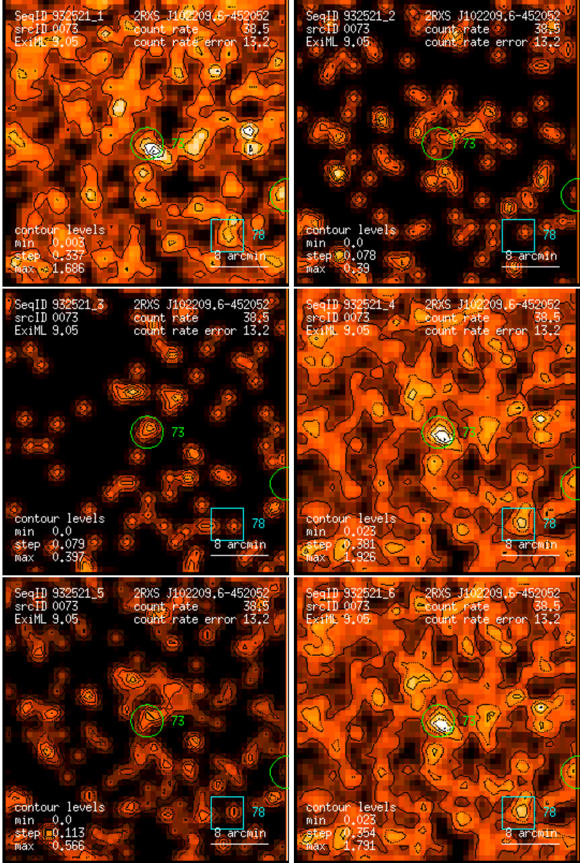
Figure 73: RASS 932521: detection 0073: band rate images, Gaussian filter: (1) PSPC channels 11 – 41, (2) 52 – 90, (3) 91 – 201, (4) 11 – 235, (5) 52 – 201, (6) 11 – 201. Broad band rates in counts/ks. Band rate contour levels in counts/ks/arcmin 2 .
