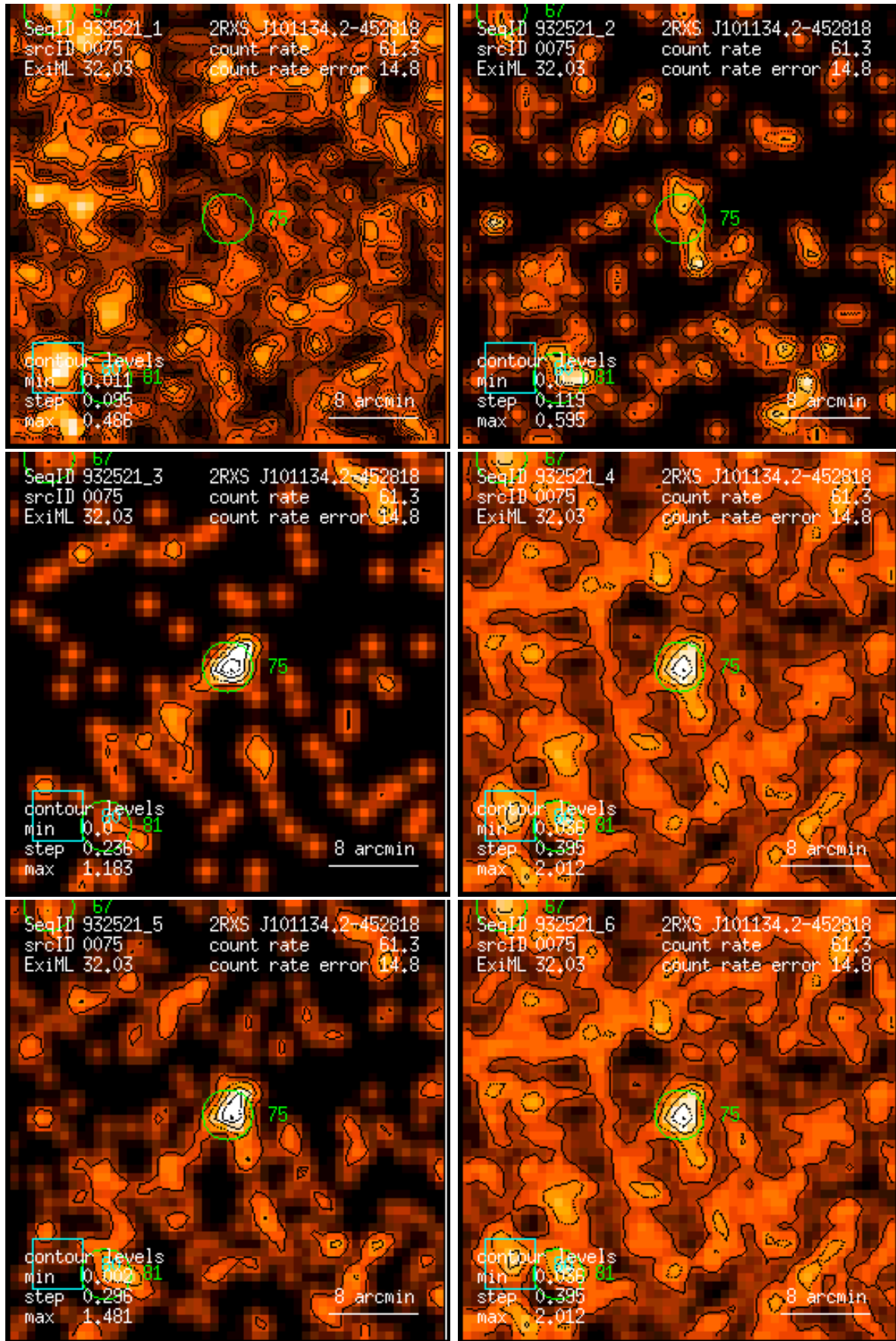
Figure 75: RASS 932521: detection 0075: band rate images, Gaussian filter: (1) PSPC channels 11 – 41, (2) 52 – 90, (3) 91 – 201, (4) 11 – 235, (5) 52 – 201, (6) 11 – 201. Broad band rates in counts/ks. Band rate contour levels in counts/ks/arcmin 2 .
