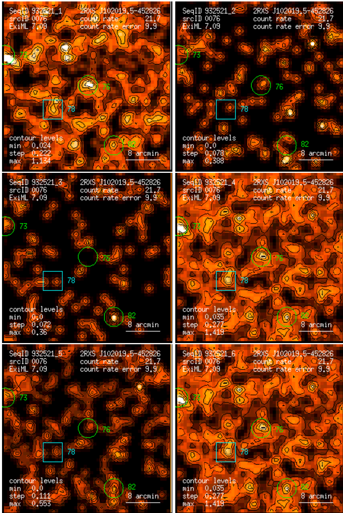
Figure 76: RASS 932521: detection 0076: band rate images, Gaussian filter: (1) PSPC channels 11 – 41, (2) 52 – 90, (3) 91 – 201, (4) 11 – 235, (5) 52 – 201, (6) 11 – 201. Broad band rates in counts/ks. Band rate contour levels in counts/ks/arcmin 2 .
