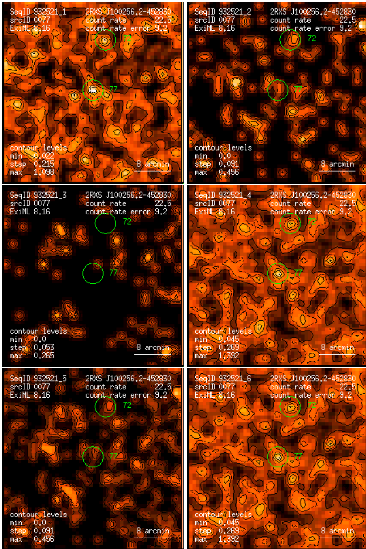
Figure 77: RASS 932521: detection 0077: band rate images, Gaussian filter: (1) PSPC channels 11 – 41, (2) 52 – 90, (3) 91 – 201, (4) 11 – 235, (5) 52 – 201, (6) 11 – 201. Broad band rates in counts/ks. Band rate contour levels in counts/ks/arcmin 2 .
