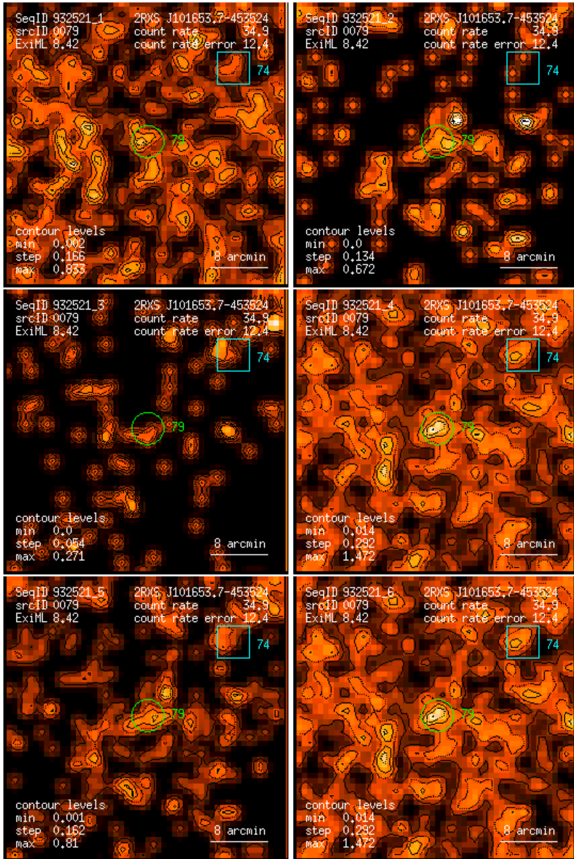
Figure 79: RASS 932521: detection 0079: band rate images, Gaussian filter: (1) PSPC channels 11 – 41, (2) 52 – 90, (3) 91 – 201, (4) 11 – 235, (5) 52 – 201, (6) 11 – 201. Broad band rates in counts/ks. Band rate contour levels in counts/ks/arcmin 2 .
