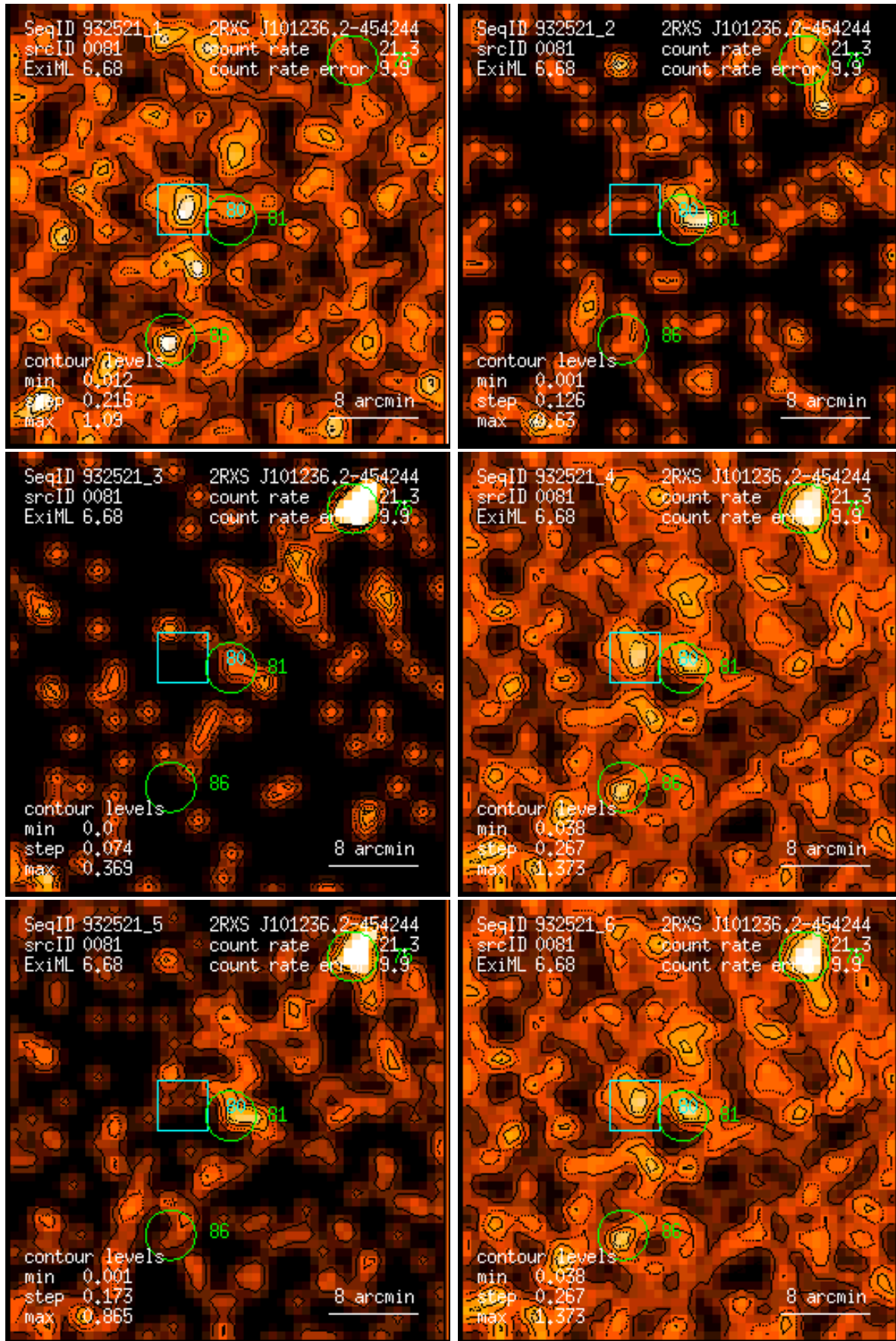
Figure 81: RASS 932521: detection 0081: band rate images, Gaussian filter: (1) PSPP channels 11 – 41, (2) 52 – 90, (3) 91 – 201, (4) 11 – 235, (5) 52 – 201, (6) 11 – 201. Broad band rates in counts/ks. Band rate contour levels in counts/ks/arcmin 2 .
