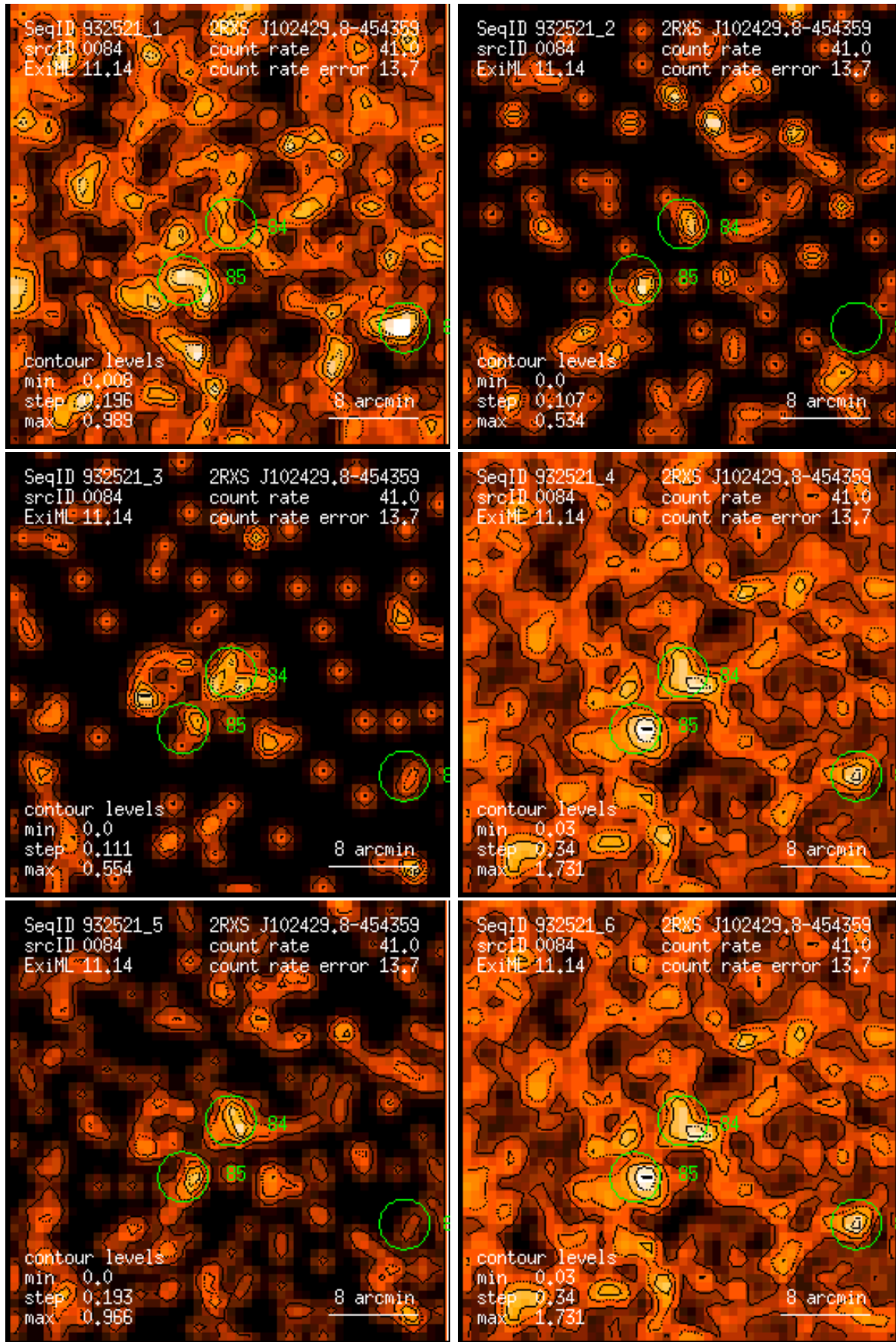
Figure 84: RASS 932521: detection 0084: band rate images, Gaussian filter: (1) PSPC channels 11 – 41, (2) 52 – 90, (3) 91 – 201, (4) 11 – 235, (5) 52 – 201, (6) 11 – 201. Broad band rates in counts/ks. Band rate contour levels in counts/ks/arcmin 2 .
