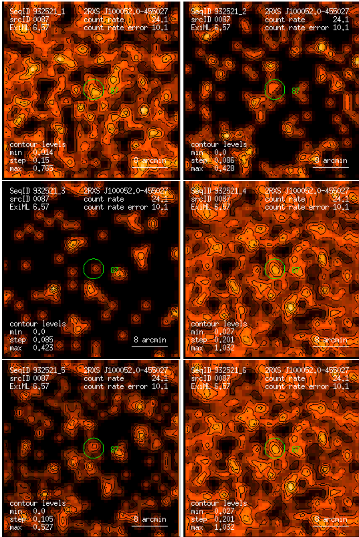
Figure 87: RASS 932521: detection 0087: band rate images, Gaussian filter: (1) PSPC channels 11 – 41, (2) 52 – 90, (3) 91 – 201, (4) 11 – 235, (5) 52 – 201, (6) 11 – 201. Broad band rates in counts/ks. Band rate contour levels in counts/ks/arcmin 2 .
