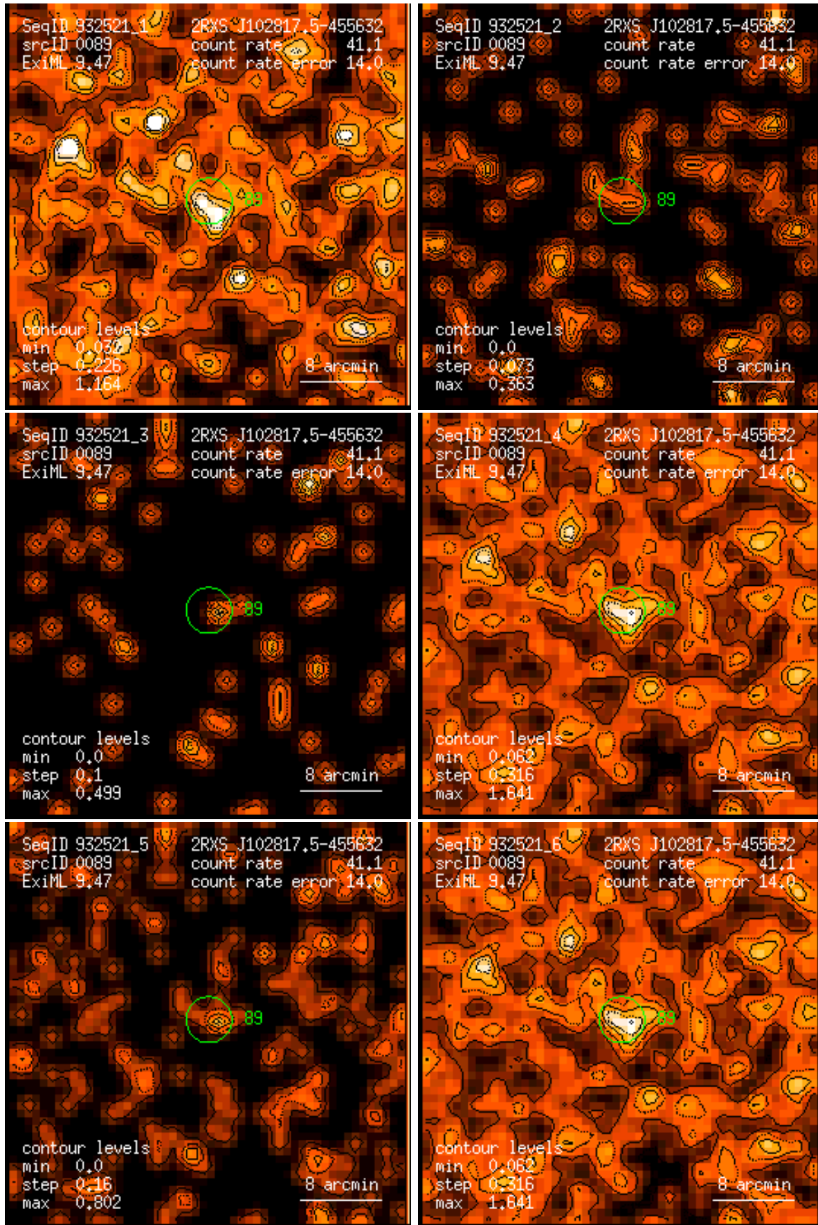
Figure 89: RASS 932521: detection 0089: band rate images, Gaussian filter: (1) PSPC channels 11 – 41, (2) 52 – 90, (3) 91 – 201, (4) 11 – 235, (5) 52 – 201, (6) 11 – 201. Broad band rates in counts/ks. Band rate contour levels in counts/ks/arcmin 2 .
