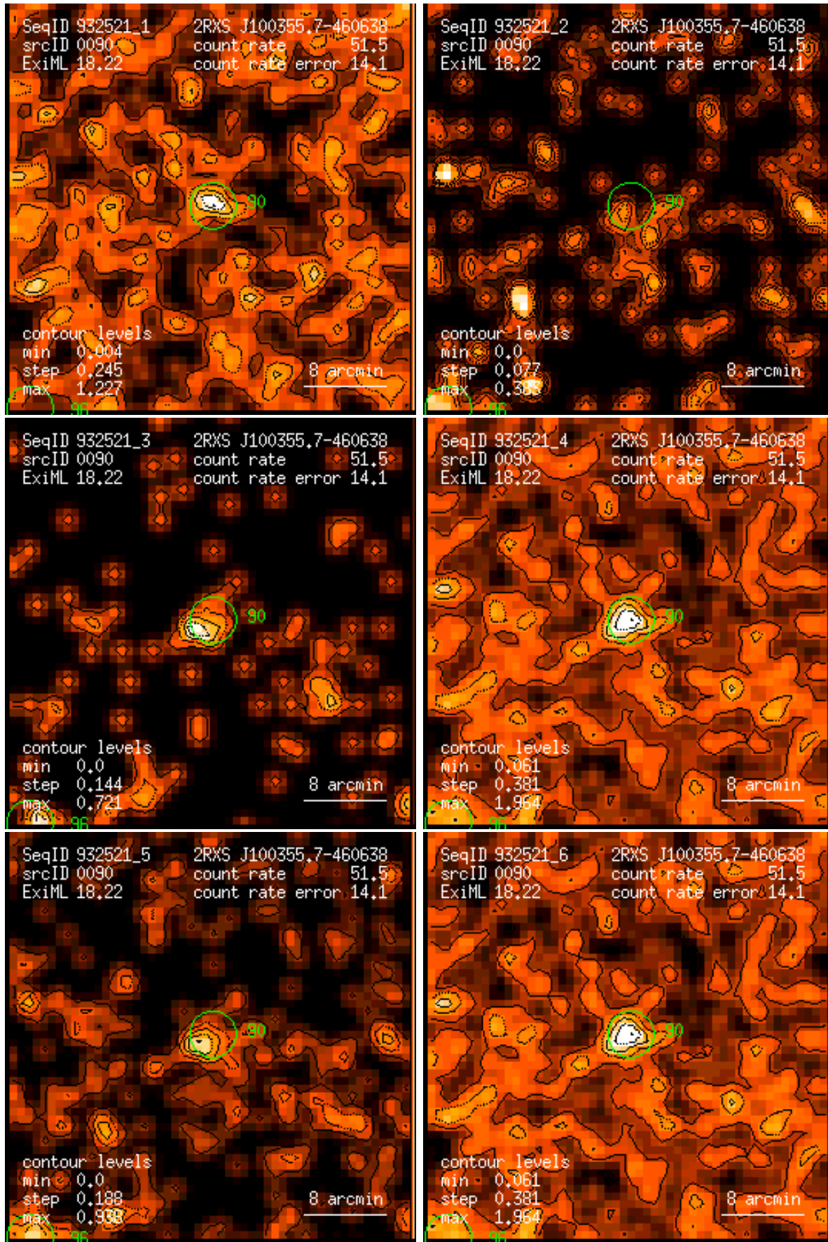
Figure 90: RASS 932521: detection 0090: band rate images, Gaussian filter: (1) PSPC channels 11 – 41, (2) 52 – 90, (3) 91 – 201, (4) 11 – 235, (5) 52 – 201, (6) 11 – 201. Broad band rates in counts/ks. Band rate contour levels in counts/ks/arcmin 2 .
