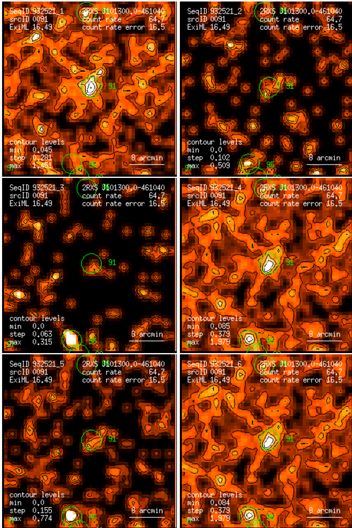
Figure 91: RASS 932521: detection 0091: band rate images, Gaussian filter: (1) PSPC channels 11 – 41, (2) 52 – 90, (3) 91 – 201, (4) 11 – 235, (5) 52 – 201, (6) 11 – 201. Broad band rates in counts/ks. Band rate contour levels in counts/ks/arcmin 2 .
