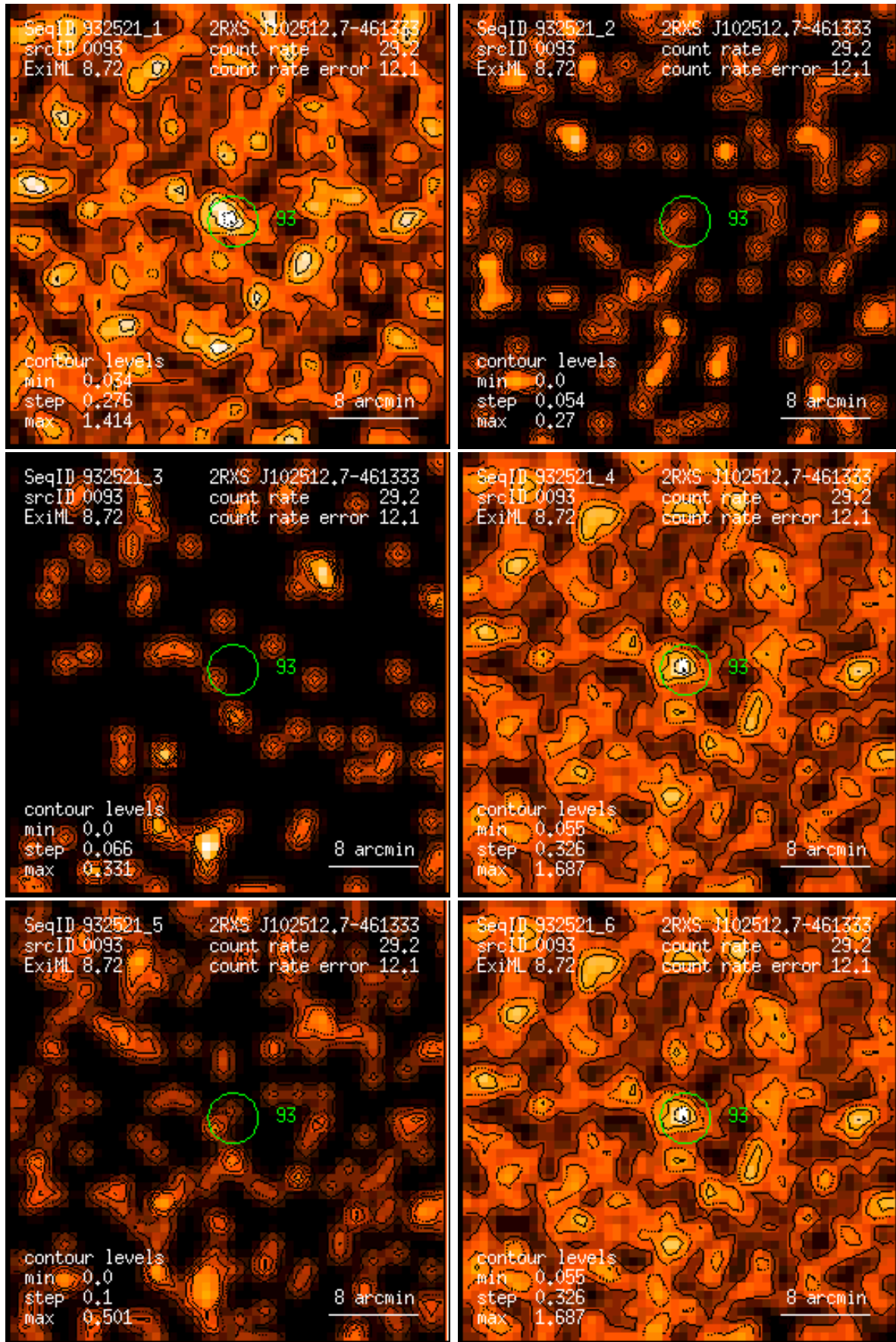
Figure 93: RASS 932521: detection 0093: band rate images, Gaussian filter: (1) PSPC channels 11 – 41, (2) 52 – 90, (3) 91 – 201, (4) 11 – 235, (5) 52 – 201, (6) 11 – 201. Broad band rates in counts/ks. Band rate contour levels in counts/ks/arcmin 2 .
