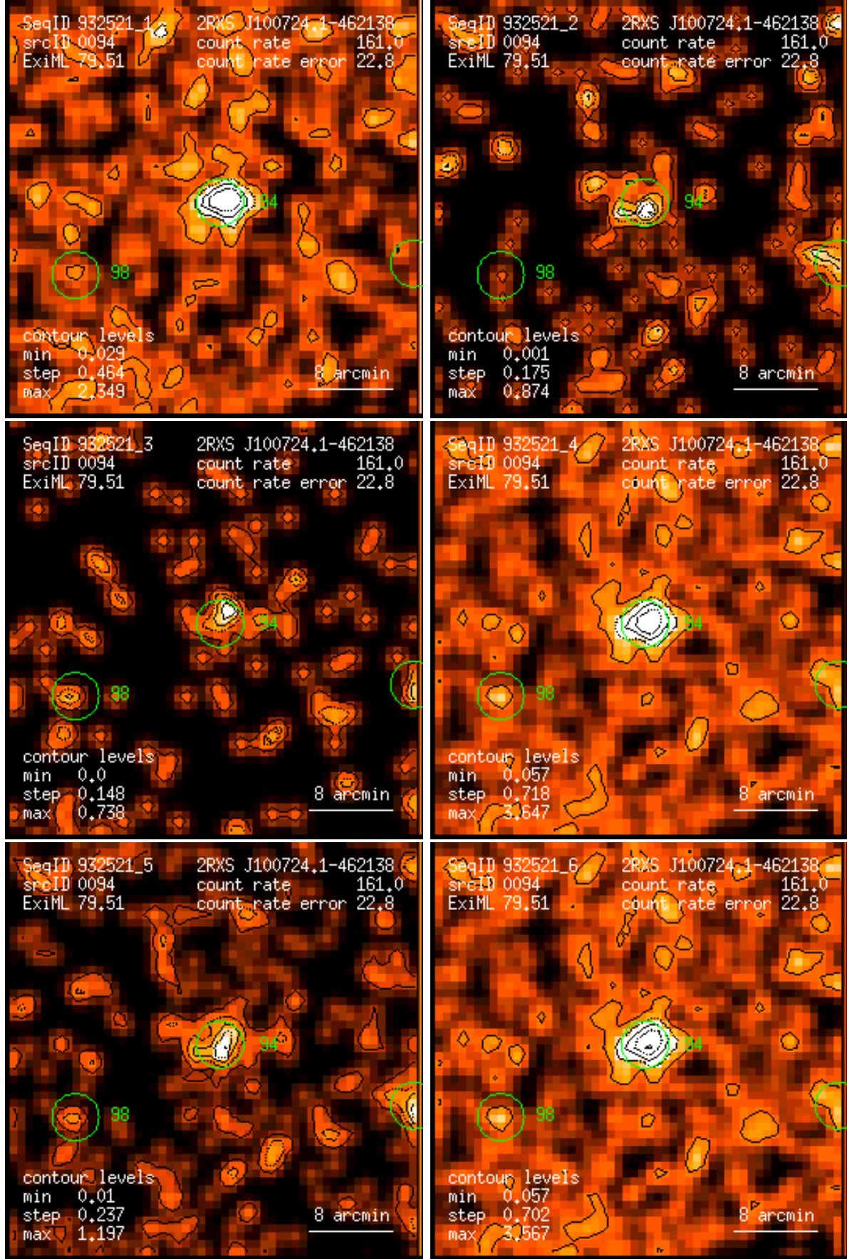
Figure 94: RASS 932521: detection 0094: band rate images, Gaussian filter: (1) PSPC channels 11 – 41, (2) 52 – 90, (3) 91 – 201, (4) 11 – 235, (5) 52 – 201, (6) 11 – 201. Broad band rates in counts/ks. Band rate contour levels in counts/ks/arcmin 2 .
