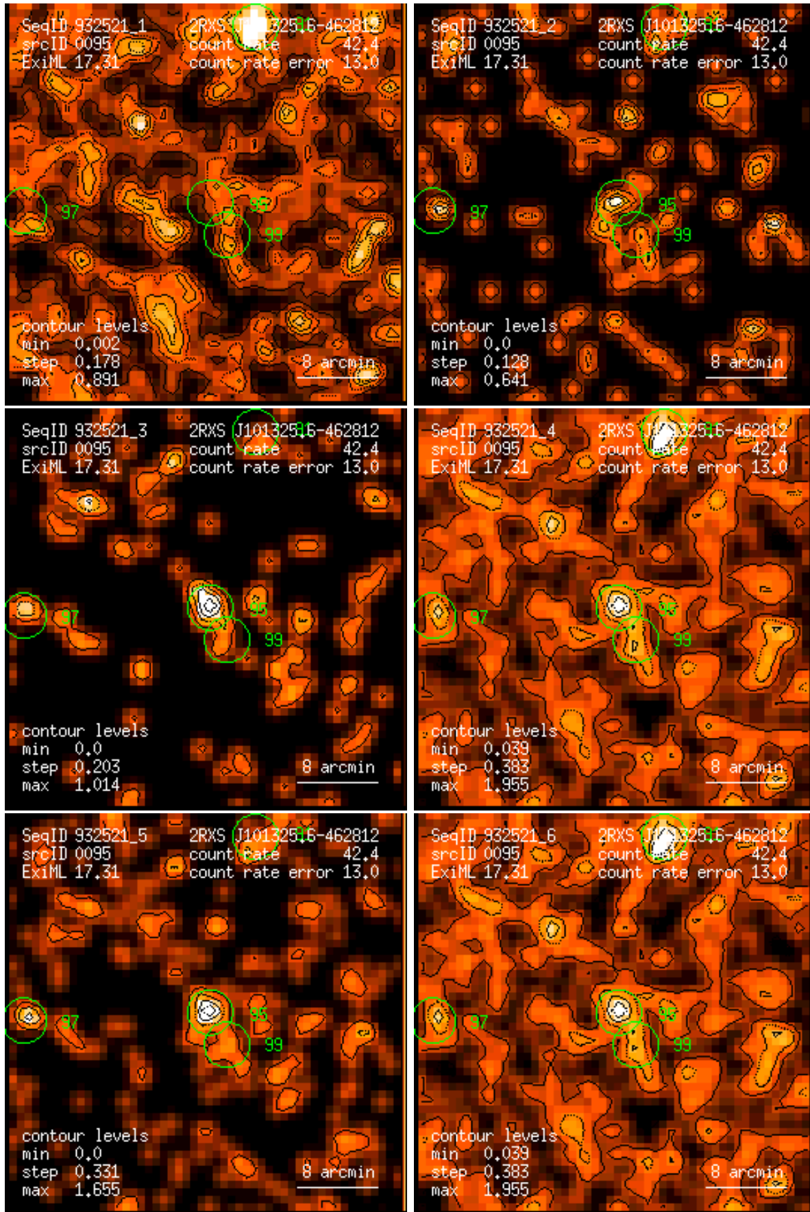
Figure 95: RASS 932521: detection 0095: band rate images, Gaussian filter: (1) PSPC channels 11 – 41, (2) 52 – 90, (3) 91 – 201, (4) 11 – 235, (5) 52 – 201, (6) 11 – 201. Broad band rates in counts/ks. Band rate contour levels in counts/ks/arcmin 2 .
