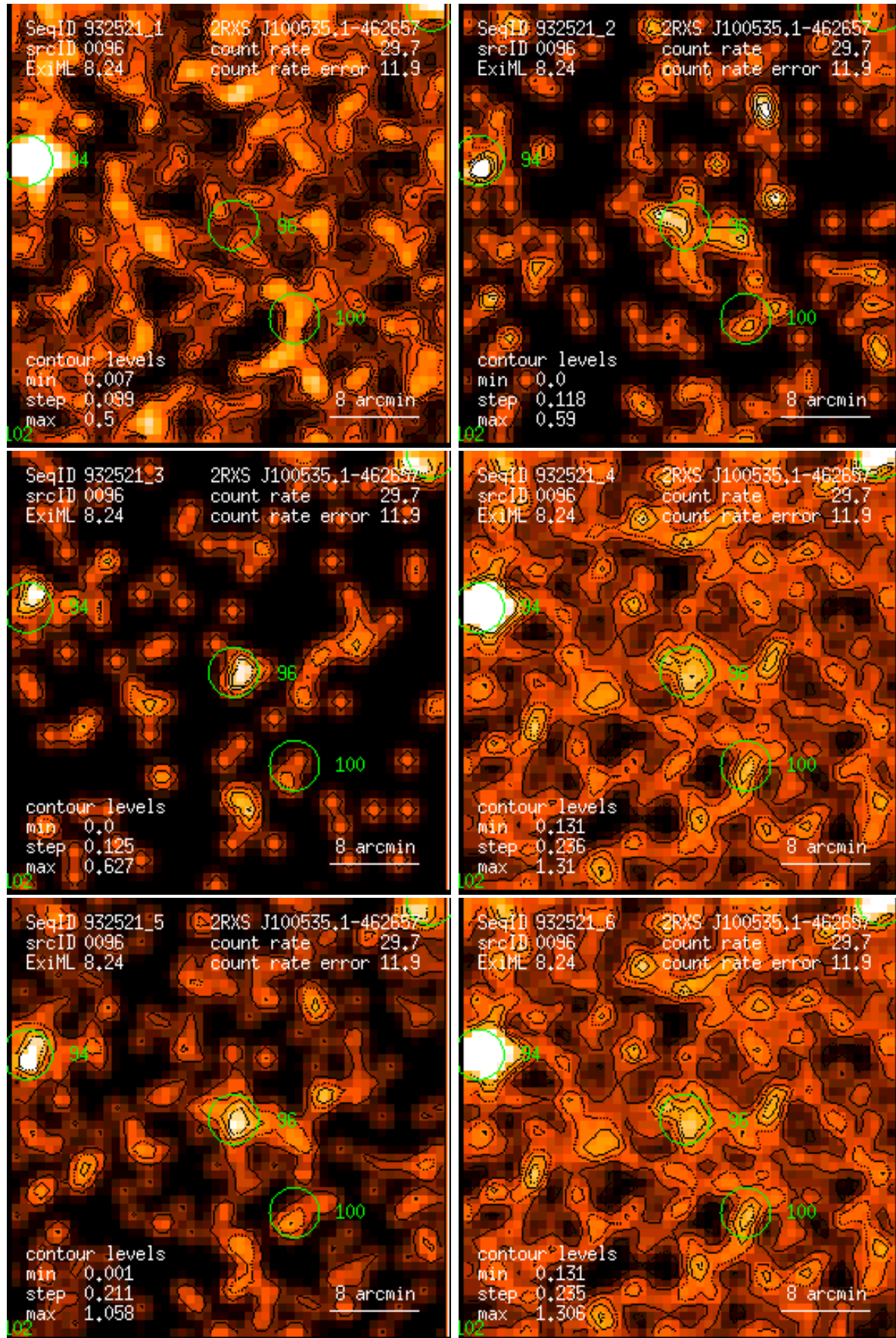
Figure 96: RASS 932521: detection 0096: band rate images, Gaussian filter: (1) PSPC channels 11 – 41, (2) 52 – 90, (3) 91 – 201, (4) 11 – 235, (5) 52 – 201, (6) 11 – 201. Broad band rates in counts/ks. Band rate contour levels in counts/ks/arcmin 2 .
