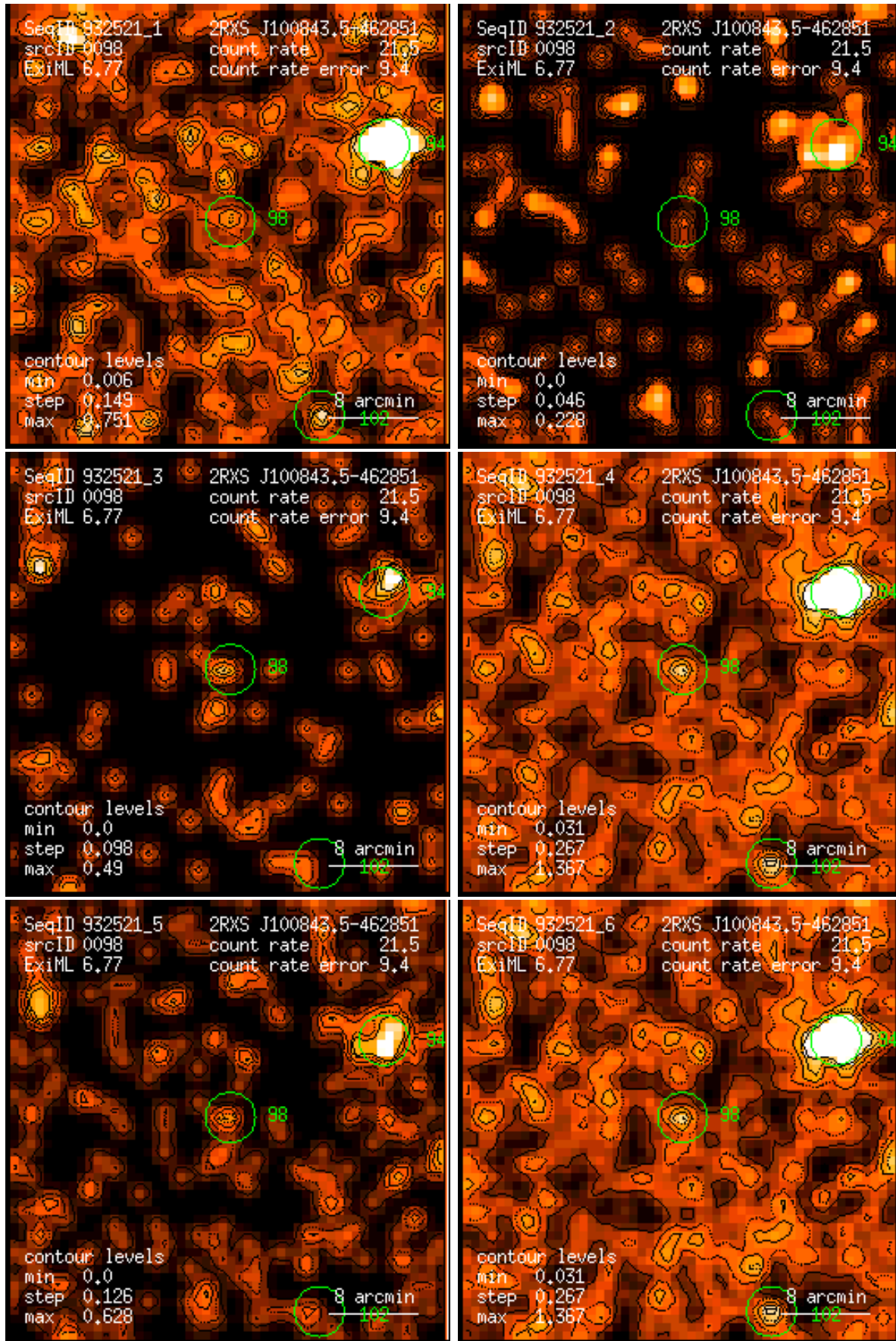
Figure 98: RASS 932521: detection 0098: band rate images, Gaussian filter: (1) PSPC channels 11 – 41, (2) 52 – 90, (3) 91 – 201, (4) 11 – 235, (5) 52 – 201, (6) 11 – 201. Broad band rates in counts/ks. Band rate contour levels in counts/ks/arcmin 2 .
