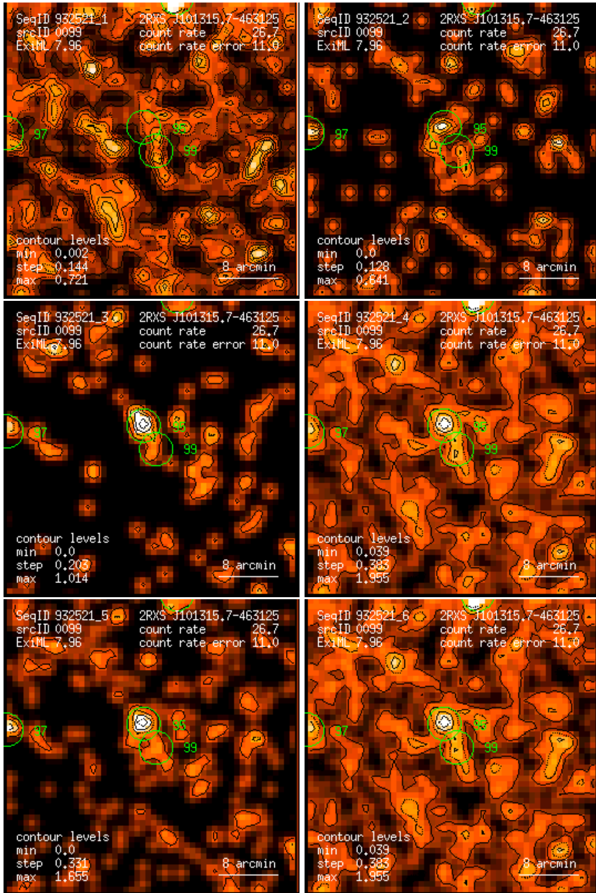
Figure 99: RASS 932521: detection 0099: band rate images, Gaussian filter: (1) PSPC channels 11 – 41, (2) 52 – 90, (3) 91 – 201, (4) 11 – 235, (5) 52 – 201, (6) 11 – 201. Broad band rates in counts/ks. Band rate contour levels in counts/ks/arcmin 2 .
