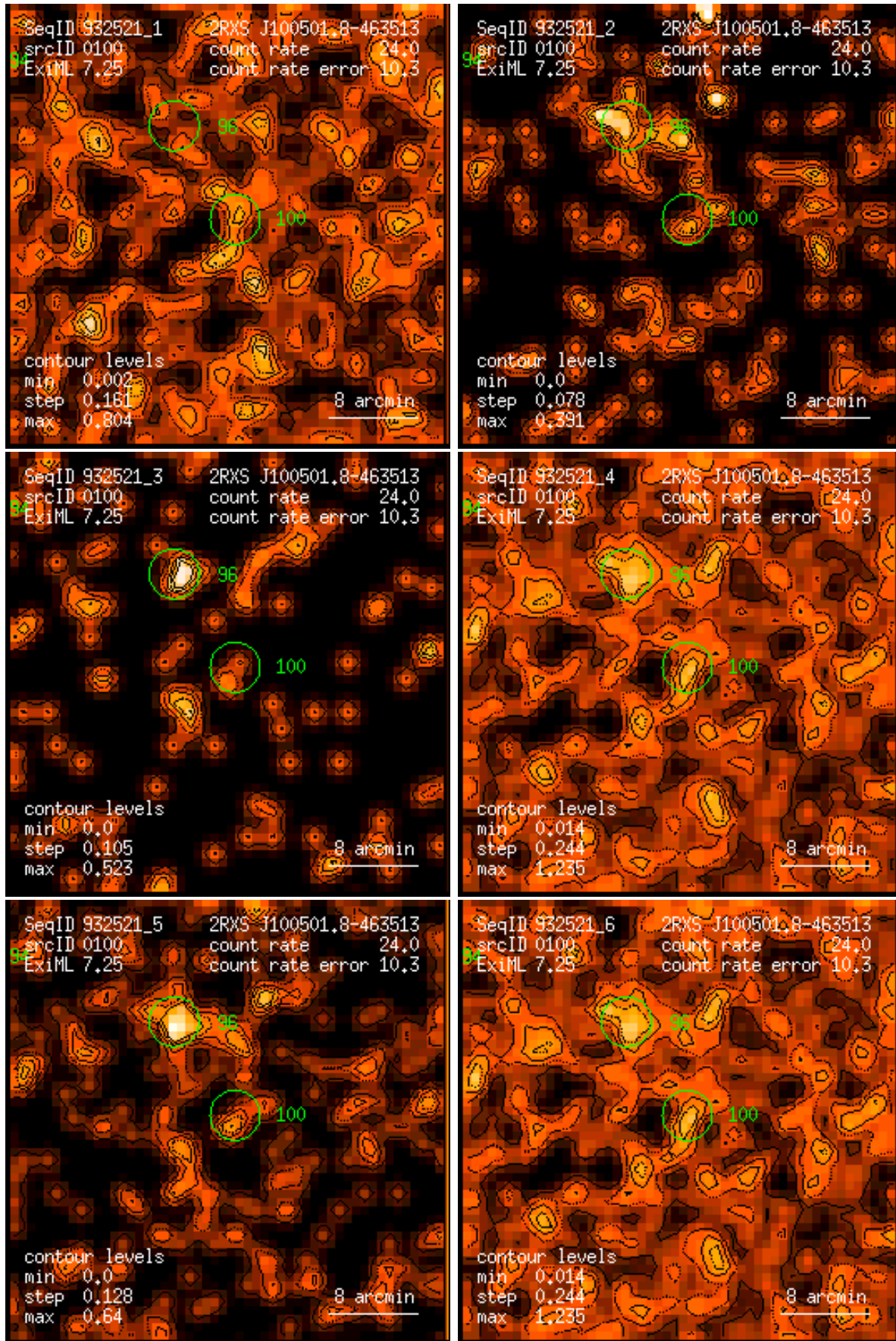
Figure 100: RASS 932521: detection 0100: band rate images, Gaussian filter: (1) PSPC channels 11 – 41, (2) 52 – 90, (3) 91 – 201, (4) 11 – 235, (5) 52 – 201, (6) 11 – 201. Broad band rates in counts/ks. Band rate contour levels in counts/ks/arcmin 2 .
