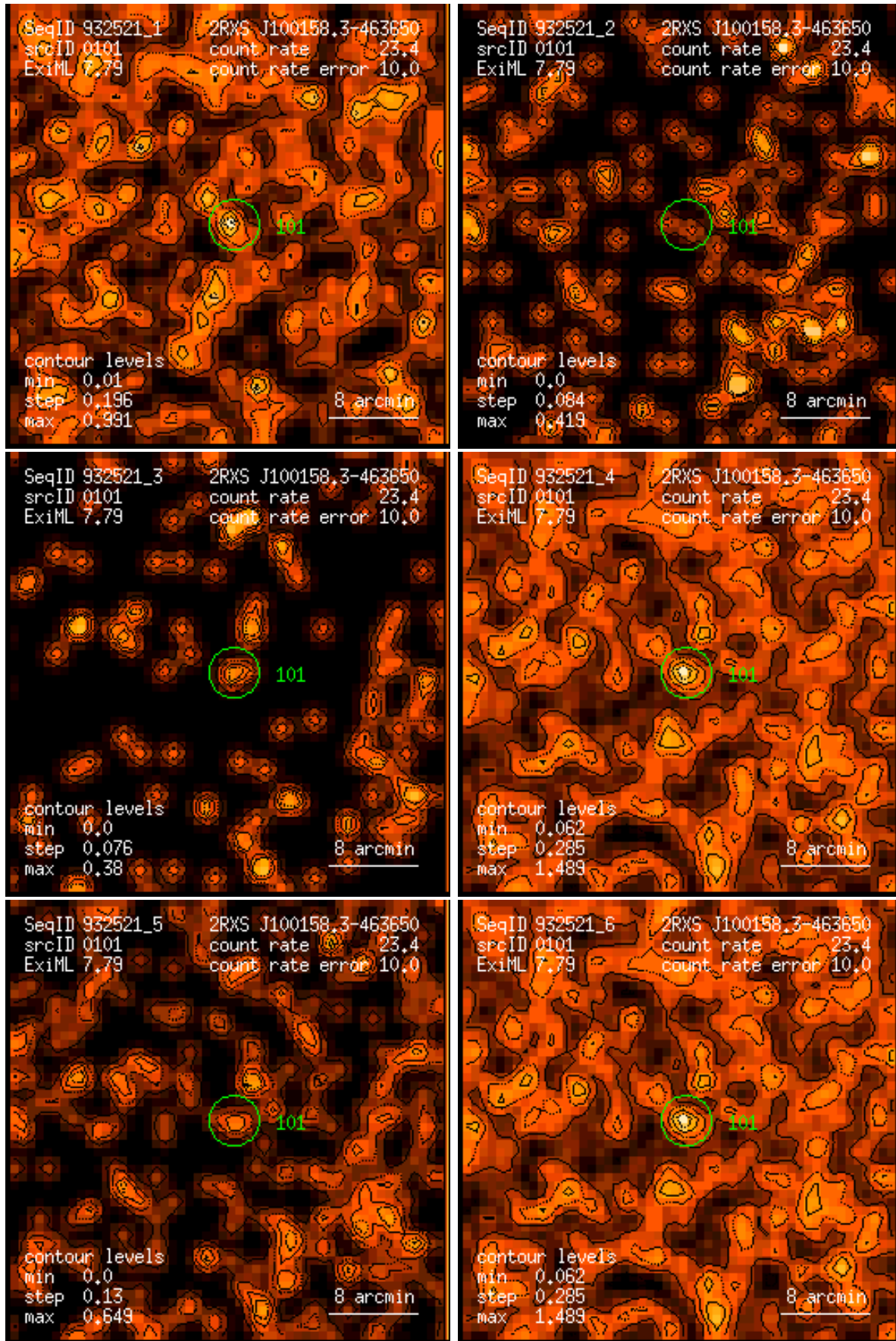
Figure 101: RASS 932521: detection 0101: band rate images, Gaussian filter: (1) PSPC channels 11 – 41, (2) 52 – 90, (3) 91 – 201, (4) 11 – 235, (5) 52 – 201, (6) 11 – 201. Broad band rates in counts/ks. Band rate contour levels in counts/ks/arcmin 2 .
