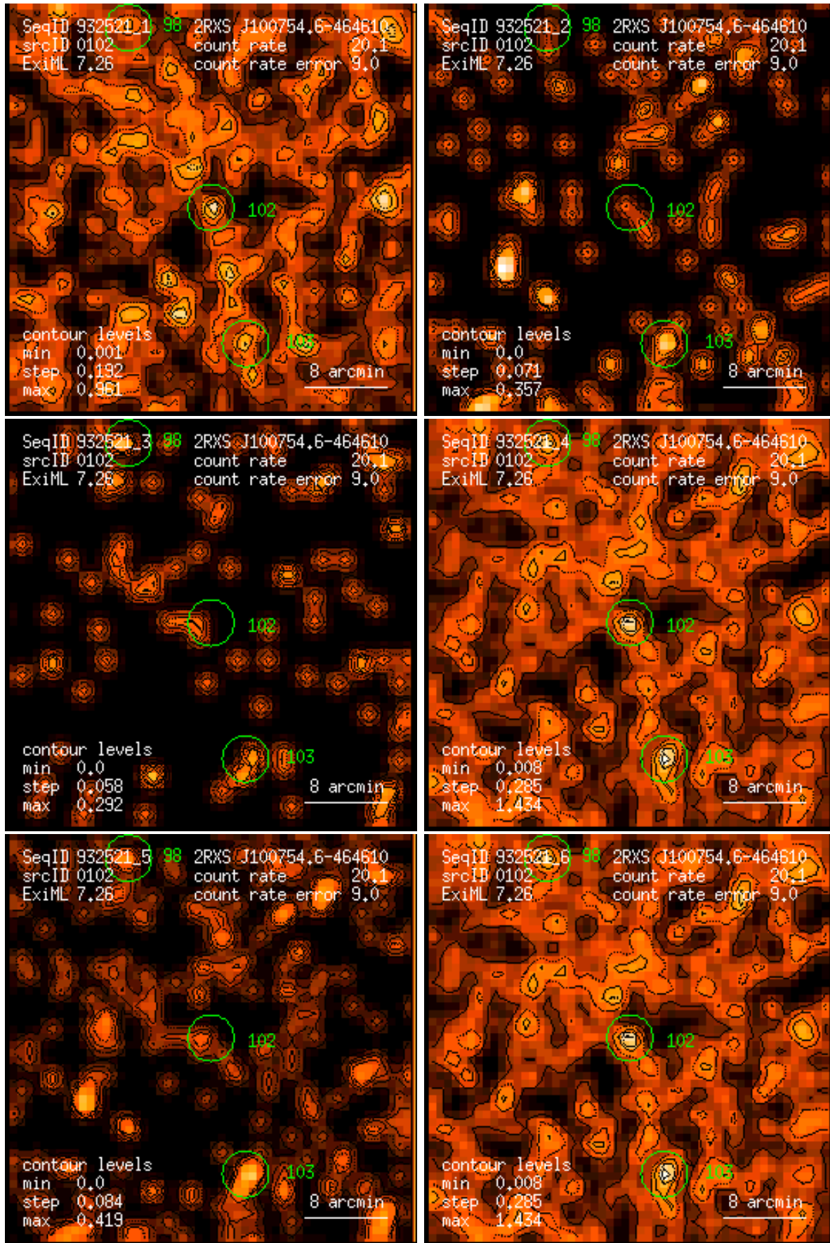
Figure 102: RASS 932521: detection 0102: band rate images, Gaussian filter: (1) PSPC channels 11 – 41, (2) 52 – 90, (3) 91 – 201, (4) 11 – 235, (5) 52 – 201, (6) 11 – 201. Broad band rates in counts/ks. Band rate contour levels in counts/ks/arcmin 2 .
