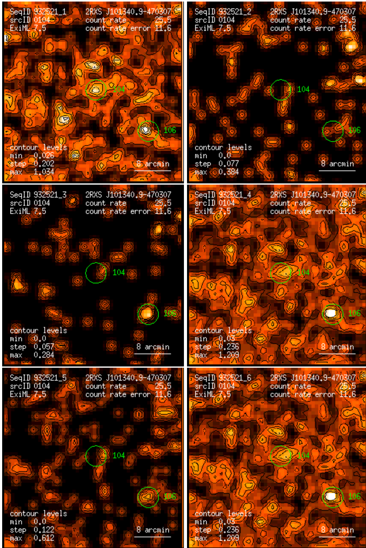
Figure 104: RASS 932521: detection 0104: band rate images, Gaussian filter: (1) PSPC channels 11 – 41, (2) 52 – 90, (3) 91 – 201, (4) 11 – 235, (5) 52 – 201, (6) 11 – 201. Broad band rates in counts/ks. Band rate contour levels in counts/ks/arcmin 2 .
