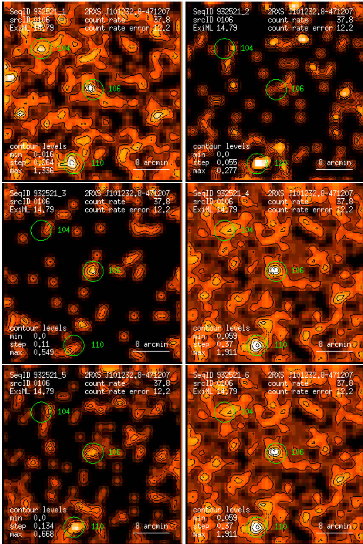
Figure 106: RASS 932521: detection 0106: band rate images, Gaussian filter: (1) PSPC channels 11 – 41, (2) 52 – 90, (3) 91 – 201, (4) 11 – 235, (5) 52 – 201, (6) 11 – 201. Broad band rates in counts/ks. Band rate contour levels in counts/ks/arcmin 2 .
