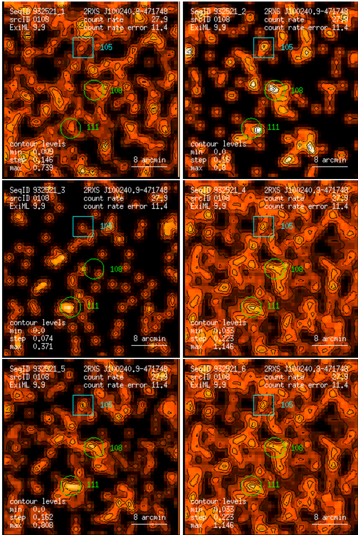
Figure 108: RASS 932521: detection 0108: band rate images, Gaussian filter: (1) PSPC channels 11 – 41, (2) 52 – 90, (3) 91 – 201, (4) 11 – 235, (5) 52 – 201, (6) 11 – 201. Broad band rates in counts/ks. Band rate contour levels in counts/ks/arcmin 2 .
