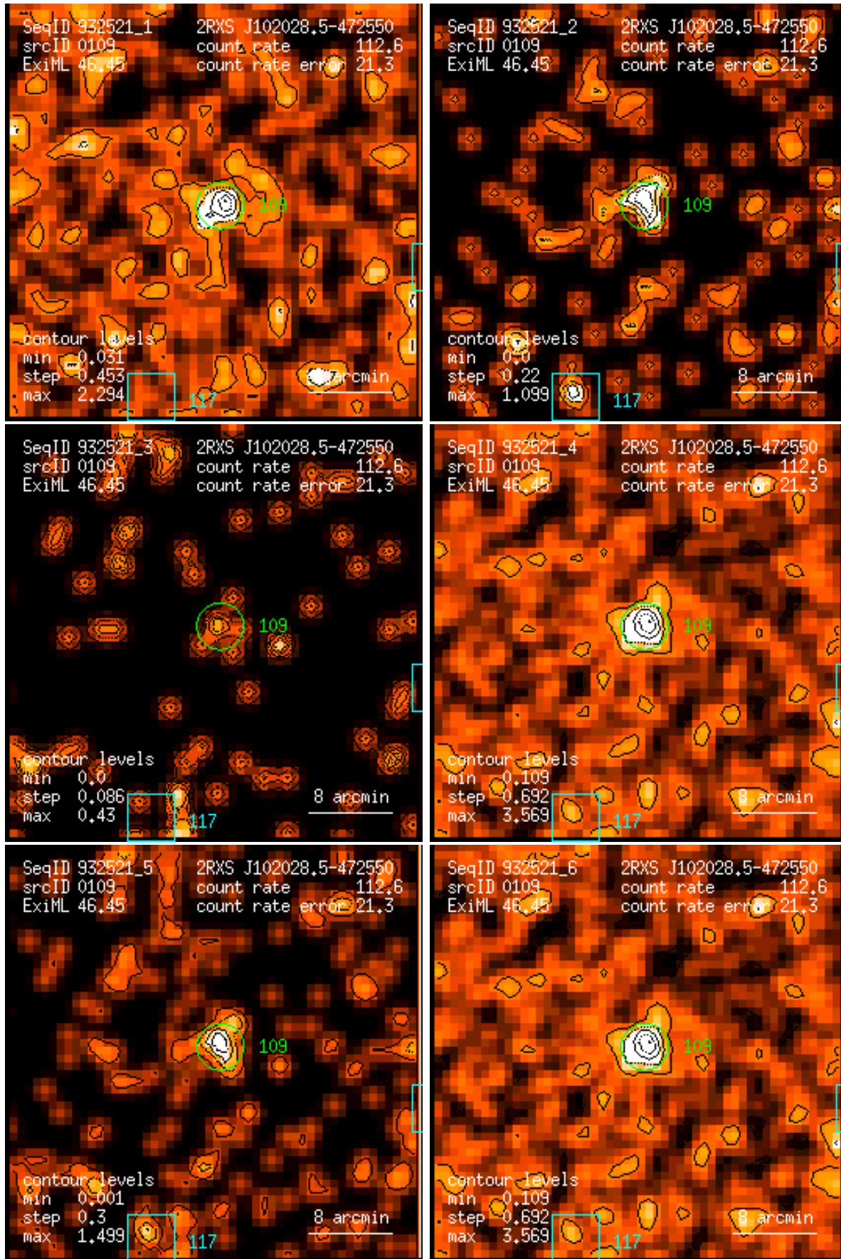
Figure 109: RASS 932521: detection 0109: band rate images, Gaussian filter: (1) PSPC channels 11 – 41, (2) 52 – 90, (3) 91 – 201, (4) 11 – 235, (5) 52 – 201, (6) 11 – 201. Broad band rates in counts/ks. Band rate contour levels in counts/ks/arcmin 2 .
