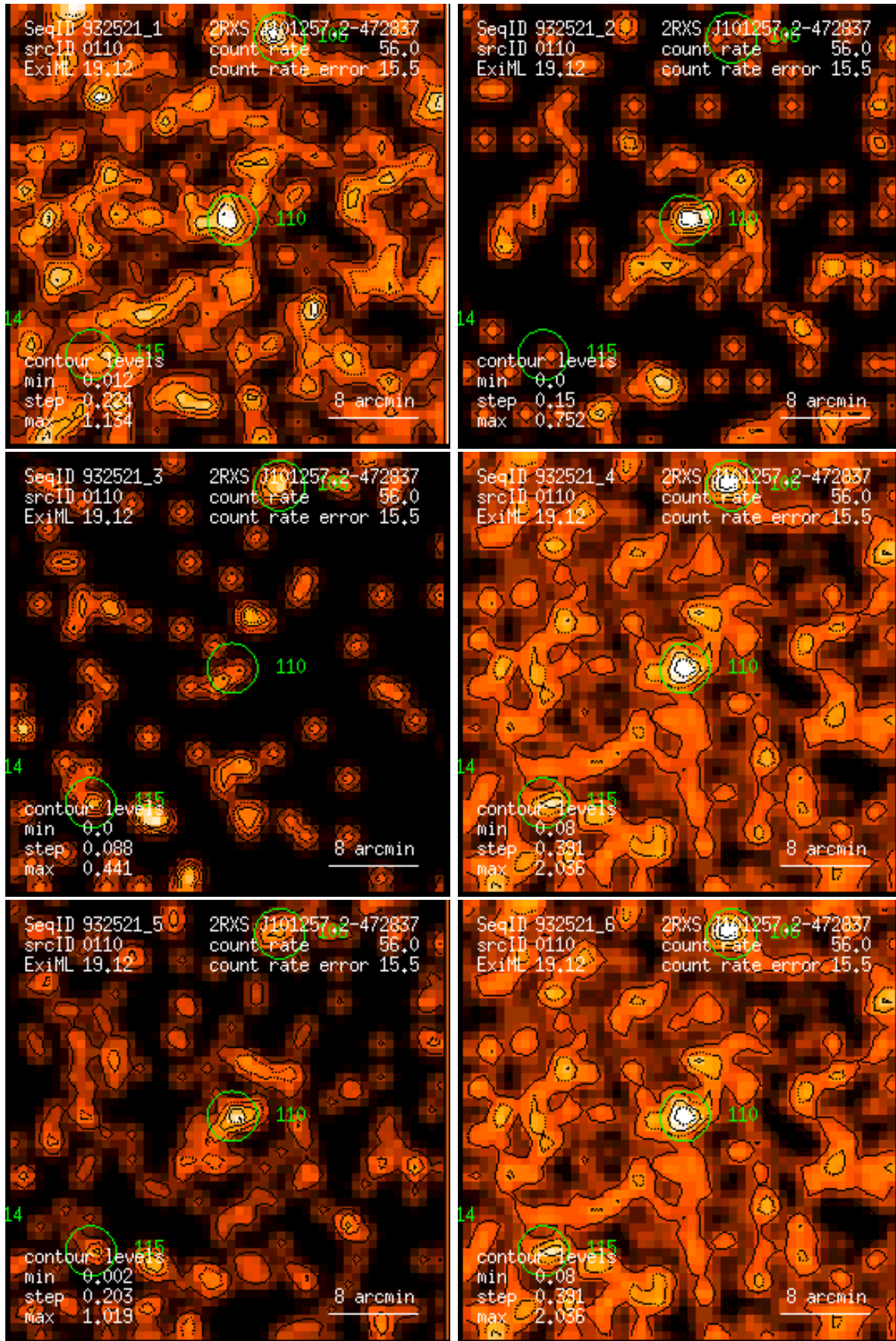
Figure 110: RASS 932521: detection 0110: band rate images, Gaussian filter: (1) PSPC channels 11 – 41, (2) 52 – 90, (3) 91 – 201, (4) 11 – 235, (5) 52 – 201, (6) 11 – 201. Broad band rates in counts/ks. Band rate contour levels in counts/ks/arcmin 2 .
