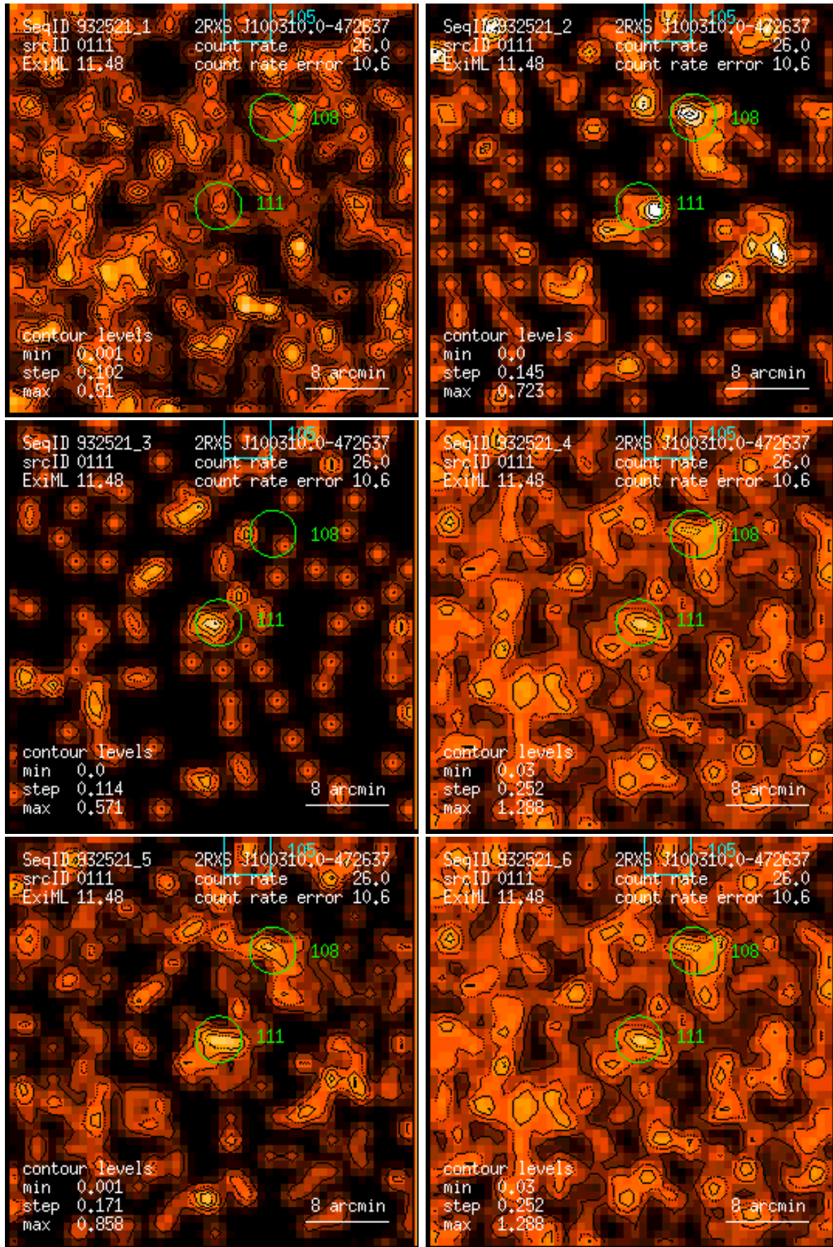
Figure 111: RASS 932521: detection 0111: band rate images, Gaussian filter: (1) PSPC channels 11 – 41, (2) 52 – 90, (3) 91 – 201, (4) 11 – 235, (5) 52 – 201, (6) 11 – 201. Broad band rates in counts/ks. Band rate contour levels in counts/ks/arcmin 2 .
