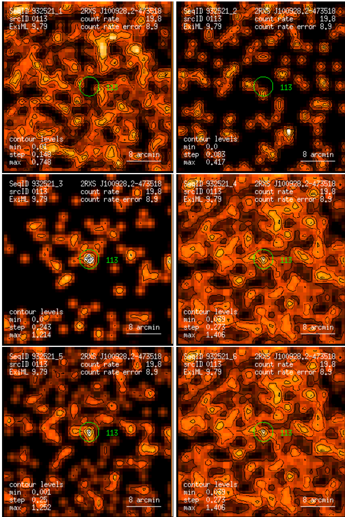
Figure 113: RASS 932521: detection 0113: band rate images, Gaussian filter: (1) PSPC channels 11 – 41, (2) 52 – 90, (3) 91 – 201, (4) 11 – 235, (5) 52 – 201, (6) 11 – 201. Broad band rates in counts/ks. Band rate contour levels in counts/ks/arcmin 2 .
