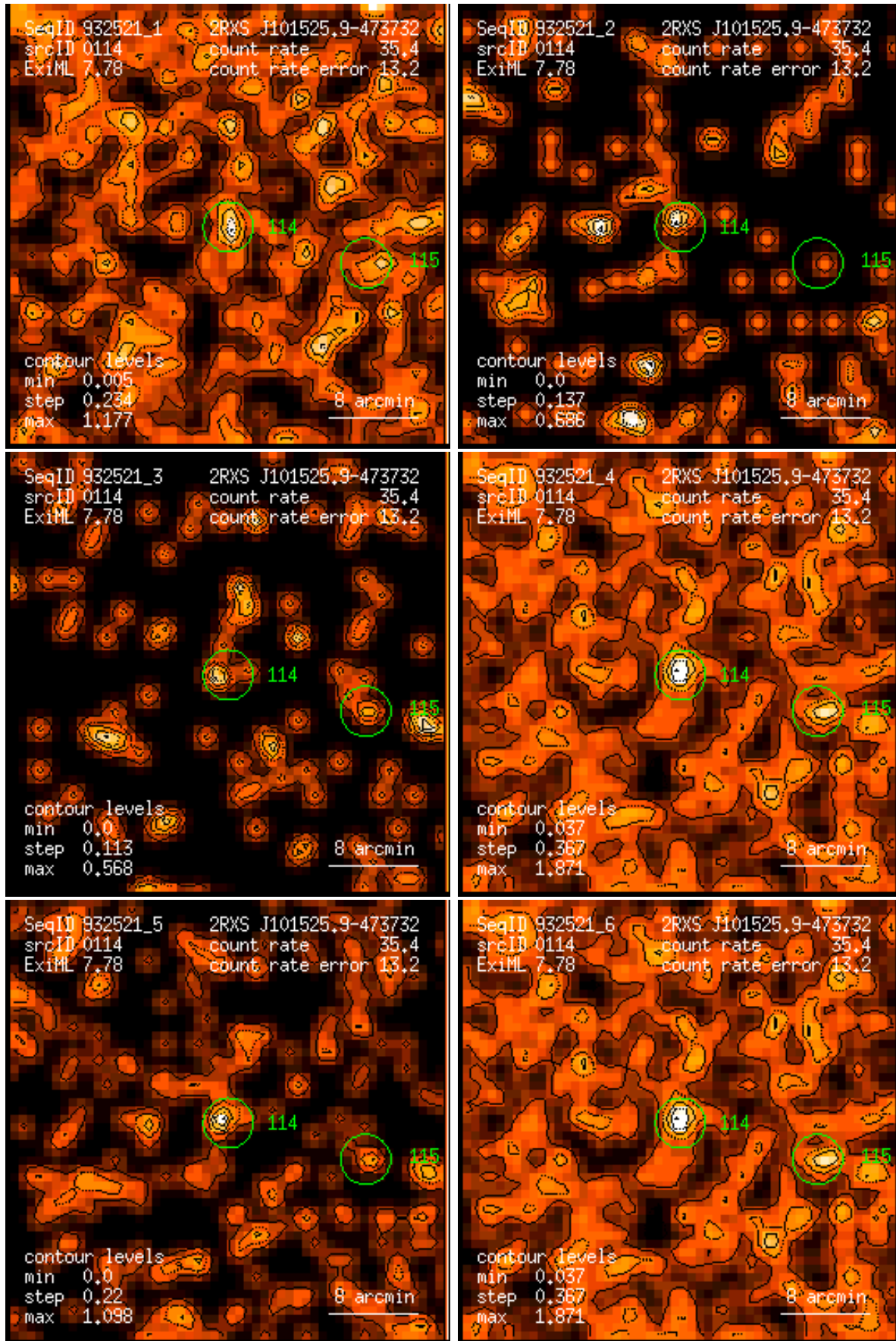
Figure 114: RASS 932521: detection 0114: band rate images, Gaussian filter: (1) PSPC channels 11 – 41, (2) 52 – 90, (3) 91 – 201, (4) 11 – 235, (5) 52 – 201, (6) 11 – 201. Broad band rates in counts/ks. Band rate contour levels in counts/ks/arcmin 2 .
