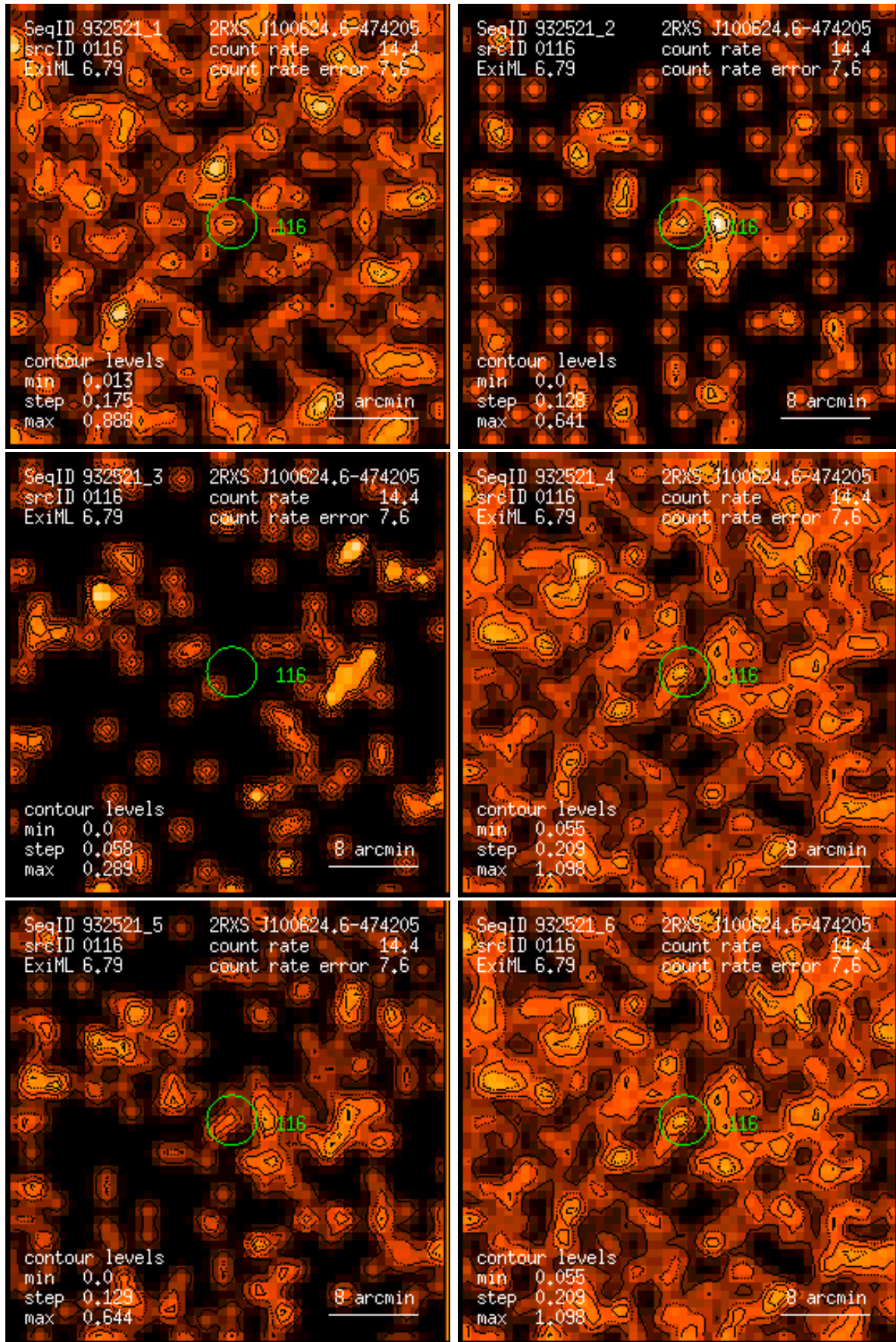
Figure 116: RASS 932521: detection 0116: band rate images, Gaussian filter: (1) PSPC channels 11 – 41, (2) 52 – 90, (3) 91 – 201, (4) 11 – 235, (5) 52 – 201, (6) 11 – 201. Broad band rates in counts/ks. Band rate contour levels in counts/ks/arcmin 2 .
