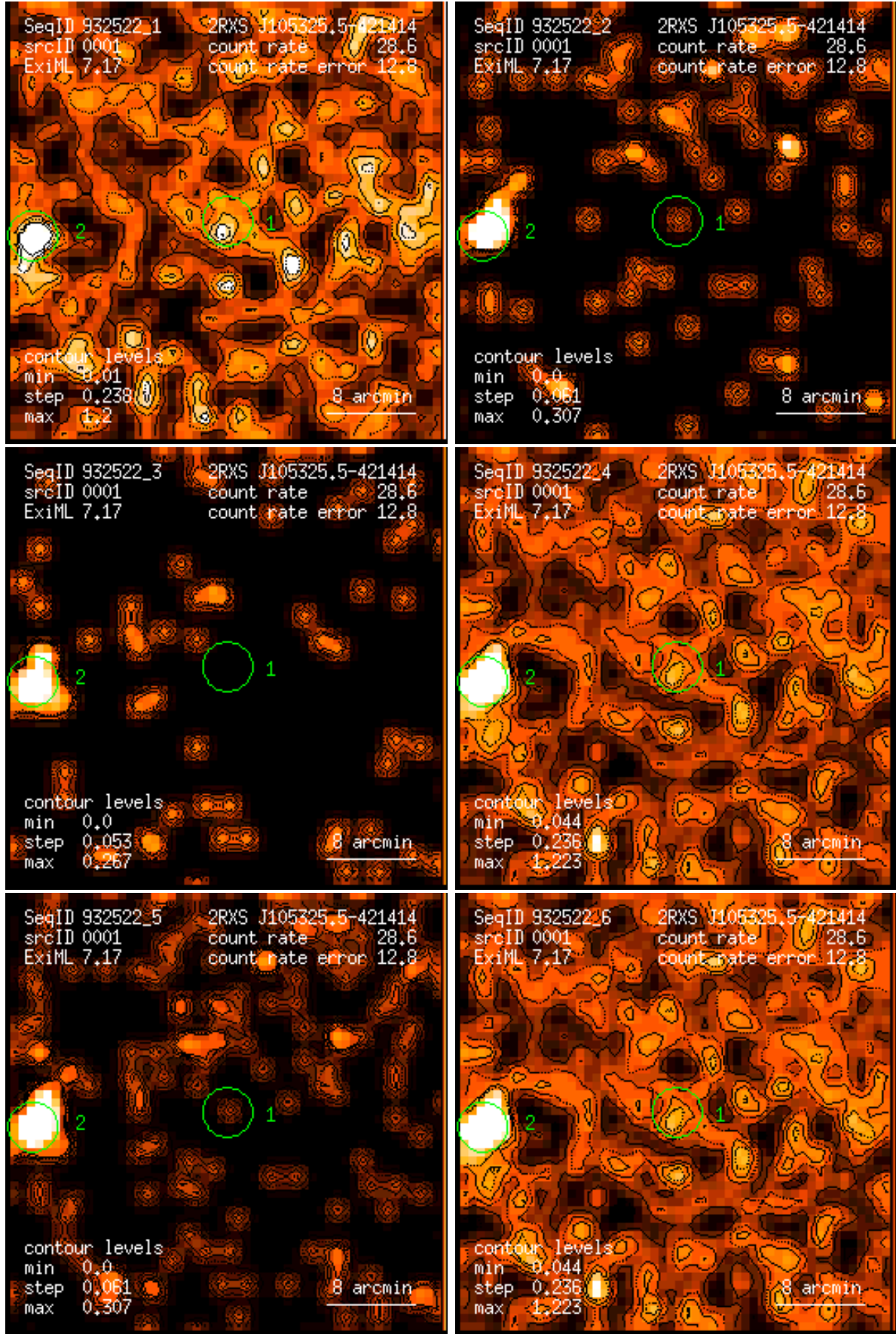
Figure 1: RASS 932522: detection 0001: band rate images, Gaussian filter: (1) PSPC channels 11 – 41, (2) 52 – 90, (3) 91 – 201, (4) 11 – 235, (5) 52 – 201, (6) 11 – 201. Broad band rates in counts/ks. Band rate contour levels in counts/ks/arcmin 2 .
