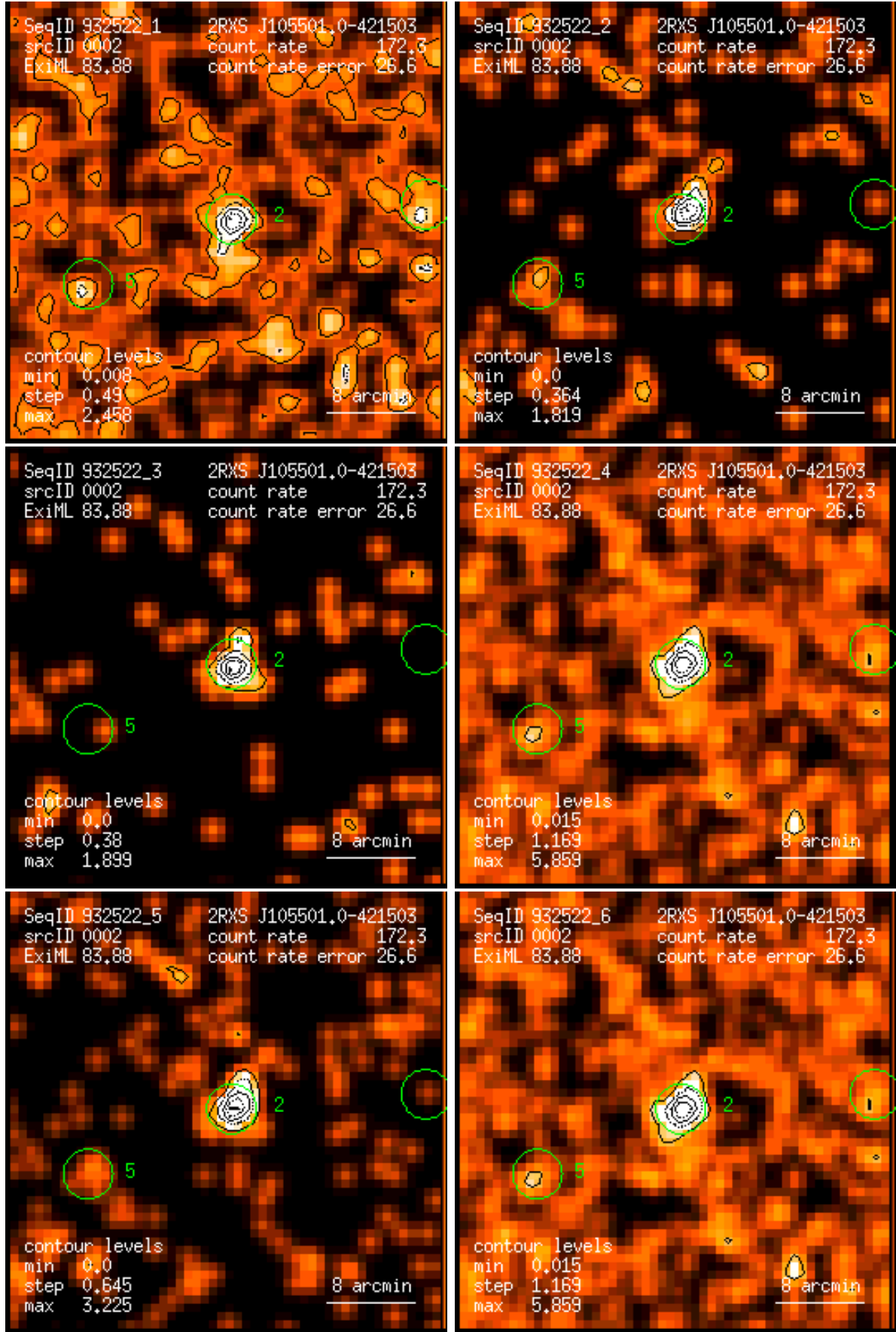
Figure 2: RASS 932522: detection 0002: band rate images, Gaussian filter: (1) PSPC channels 11 – 41, (2) 52 – 90, (3) 91 – 201, (4) 11 – 235, (5) 52 – 201, (6) 11 – 201. Broad band rates in counts/ks. Band rate contour levels in counts/ks/arcmin 2 .
