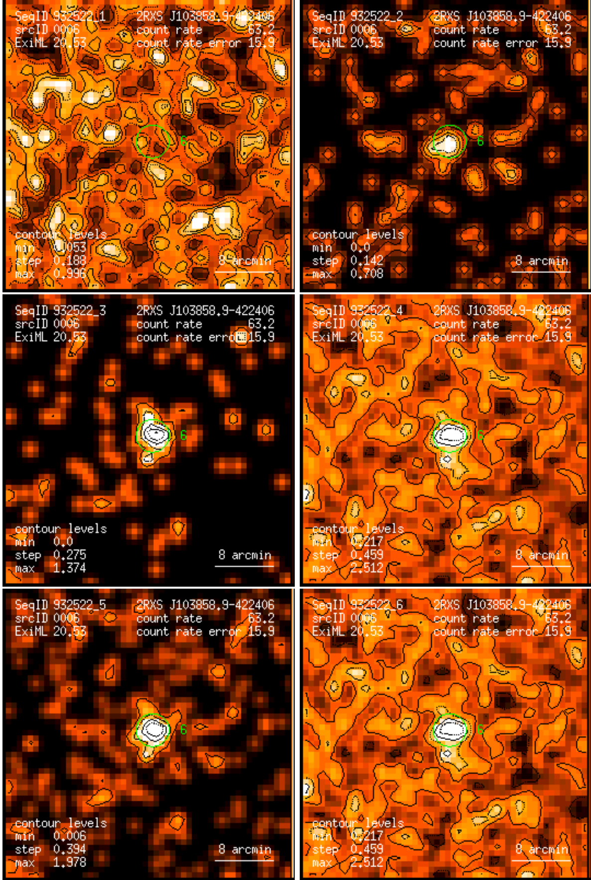
Figure 6: RASS 932522: detection 0006: band rate images, Gaussian filter: (1) PSPC channels 11 – 41, (2) 52 – 90, (3) 91 – 201, (4) 11 – 235, (5) 52 – 201, (6) 11 – 201. Broad band rates in counts/ks. Band rate contour levels in counts/ks/arcmin 2 .
