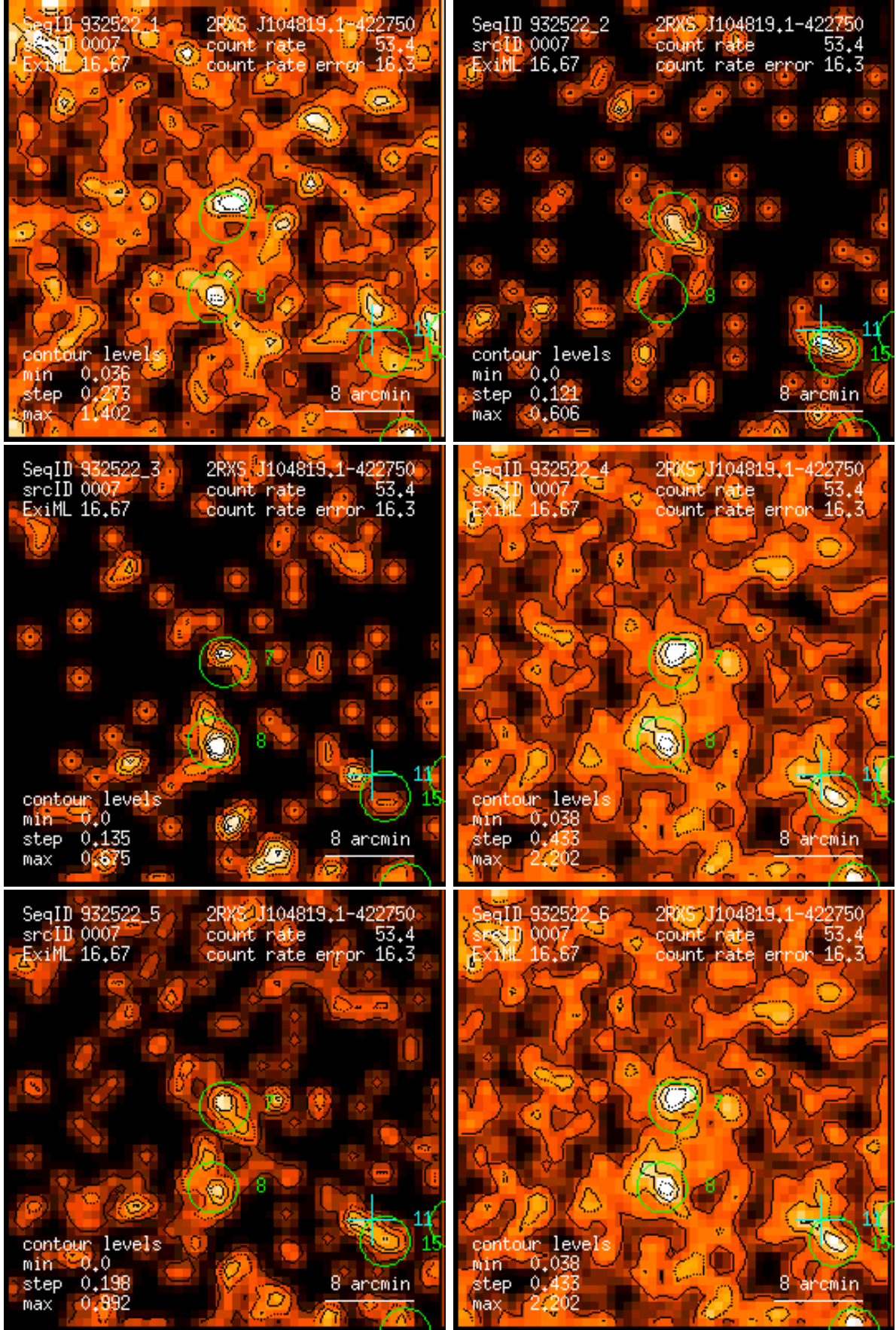
Figure 7: RASS 932522: detection 0007: band rate images, Gaussian filter: (1) PSPC channels 11 – 41, (2) 52 – 90, (3) 91 – 201, (4) 11 – 235, (5) 52 – 201, (6) 11 – 201. Broad band rates in counts/ks. Band rate contour levels in counts/ks/arcmin 2 .
